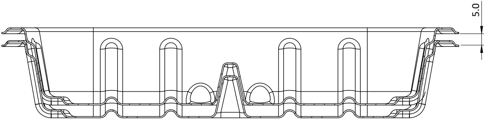
SECTION VIEW - (A - B STACKING)
