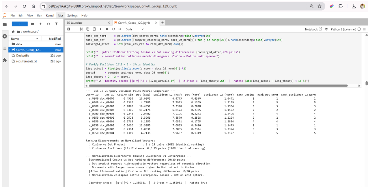
Figure 3a: Task 3 metric comparison table. Normalized cosine, dot product, and L2 rankings agree across the sampled query-document pairs.
