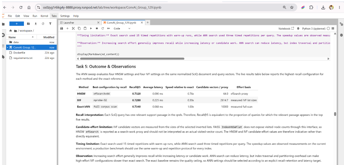
Figure 5c: Task 5 outcome and observations. It identifies the best configurations per method and prepares the decision logic used in Task 6.
