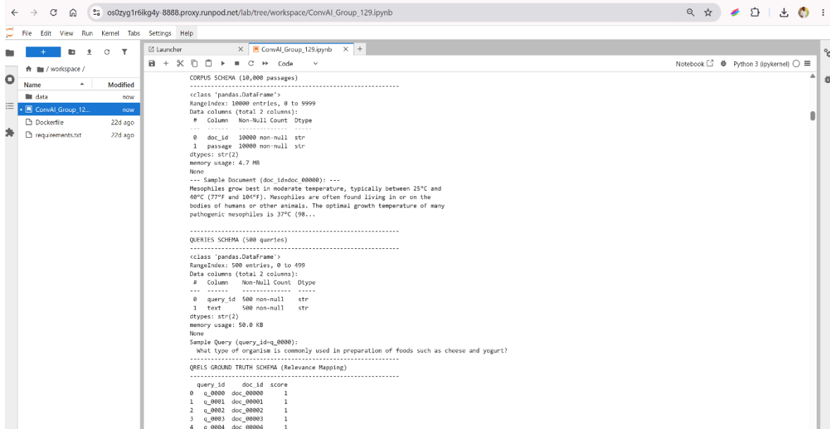
Figure 1b: Task 1 schema inspection. The visible records confirm that document IDs, query IDs, and relevance mappings are aligned for retrieval evaluation.
