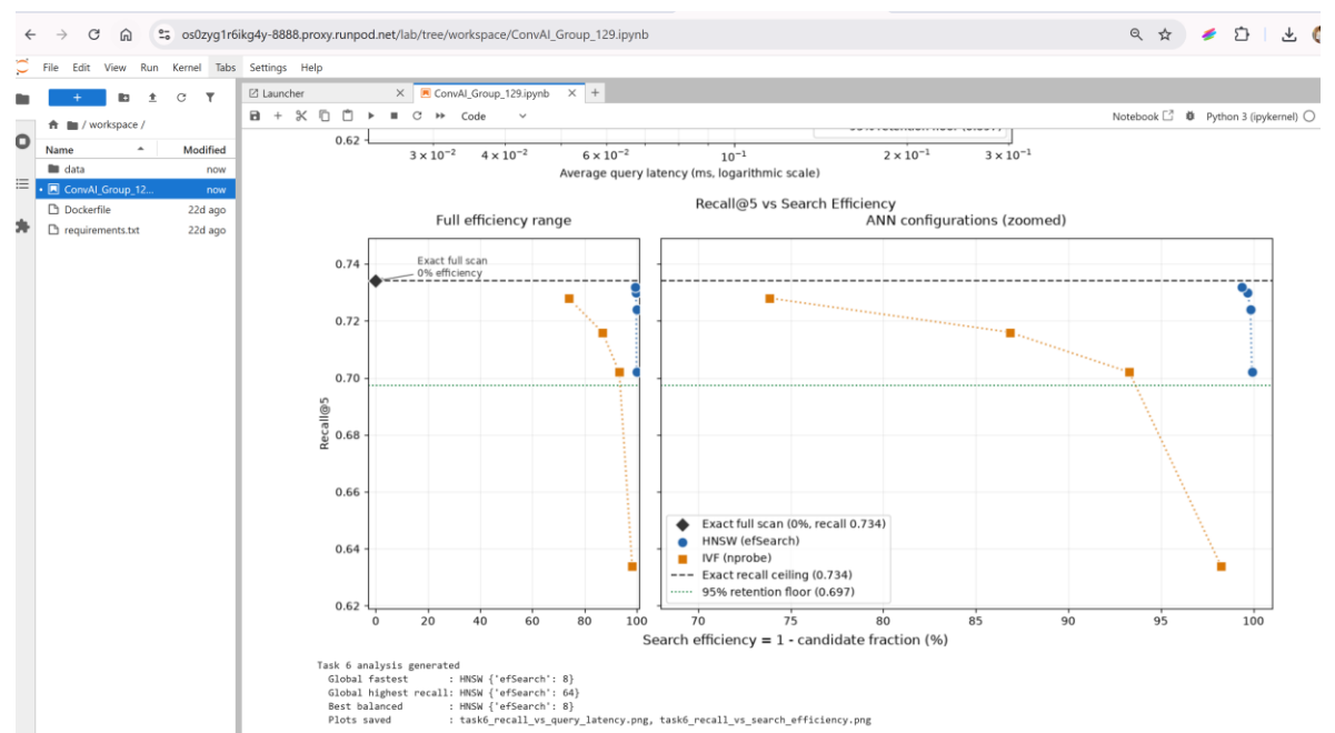
Figure 6e: Task 6 supporting search-efficiency artifact. It helps justify why efficiency should be interpreted differently for HNSW and IVF.
