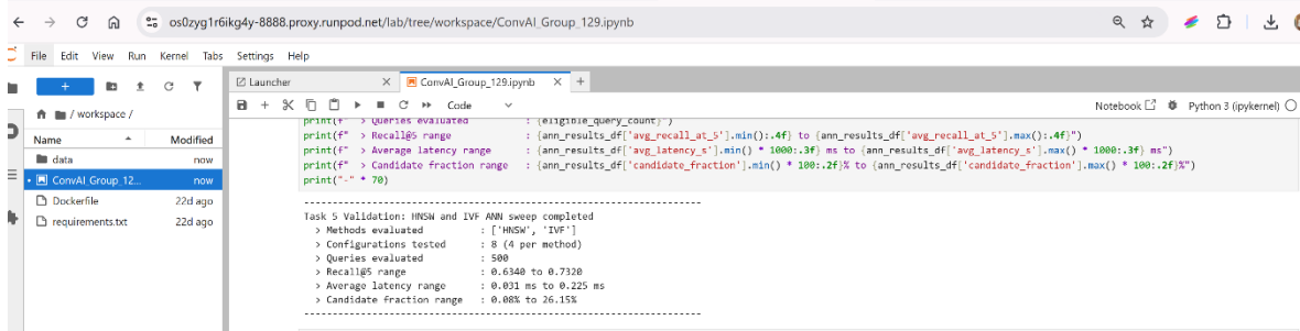
Figure 5b: Task 5 validation summary. The validation confirms complete sweep coverage and valid recall, latency, and candidate-effort ranges.
