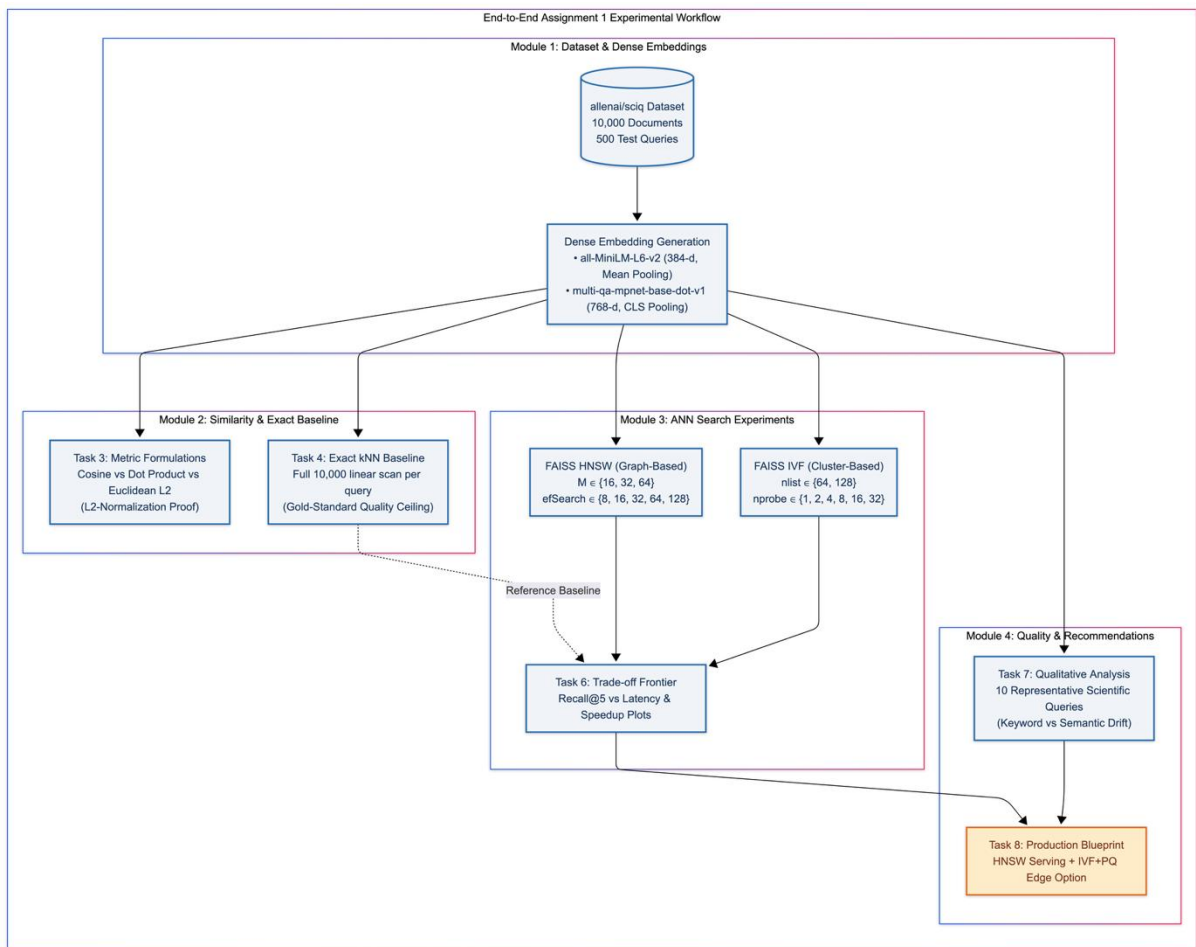
Figure 1: End-to-End Experimental Methodology and Evaluation Pipeline for SciQ Semantic Retrieval. It shows how the report modules connect, so later task-specific figures can be read as parts of one evaluation pipeline.
