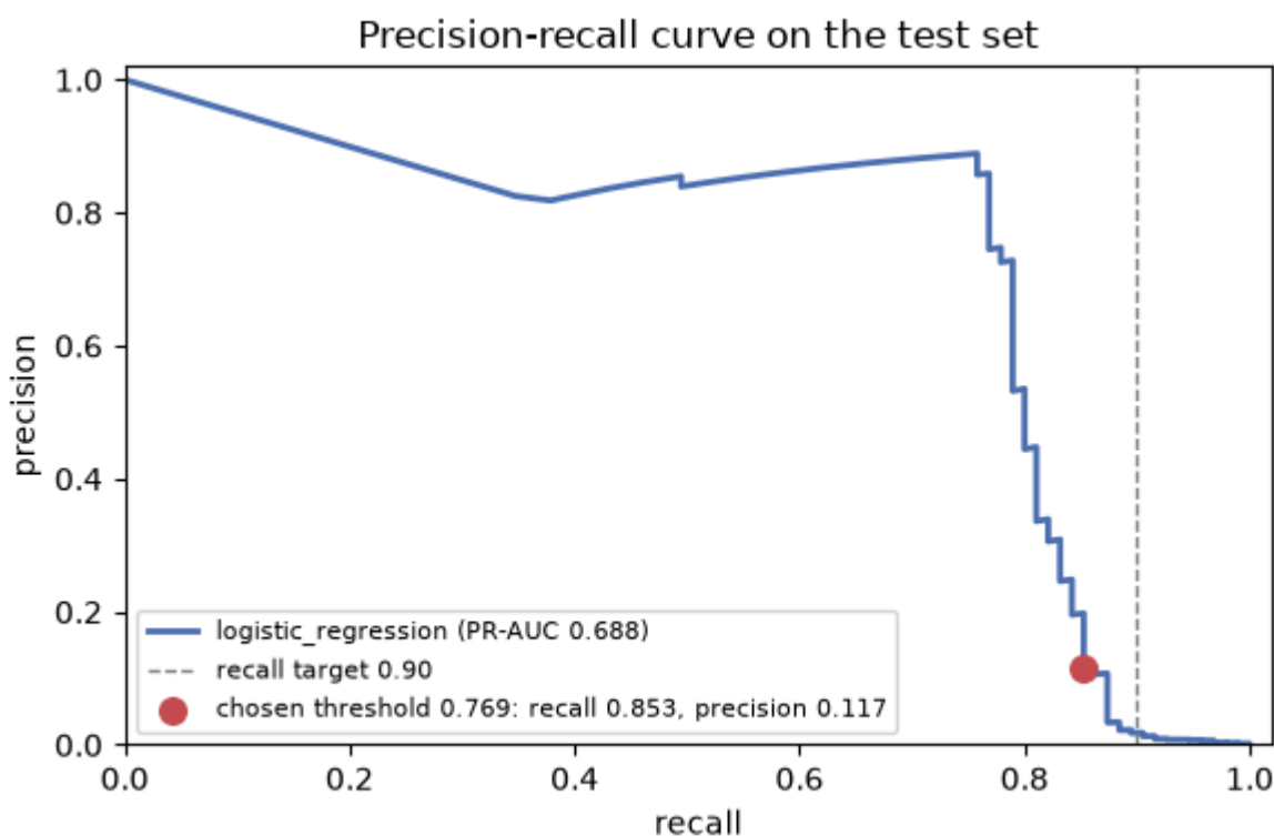
Figure 7 - Precision-recall curve on the test set. The red point is the threshold chosen on validation (0.769), which gives recall 0.853 and precision 0.117 on the test set. The dashed line is the 90% recall target. Reaching it on this test set would lower precision to 1.8%, with 4,690 genuine transactions flagged instead of 612.
