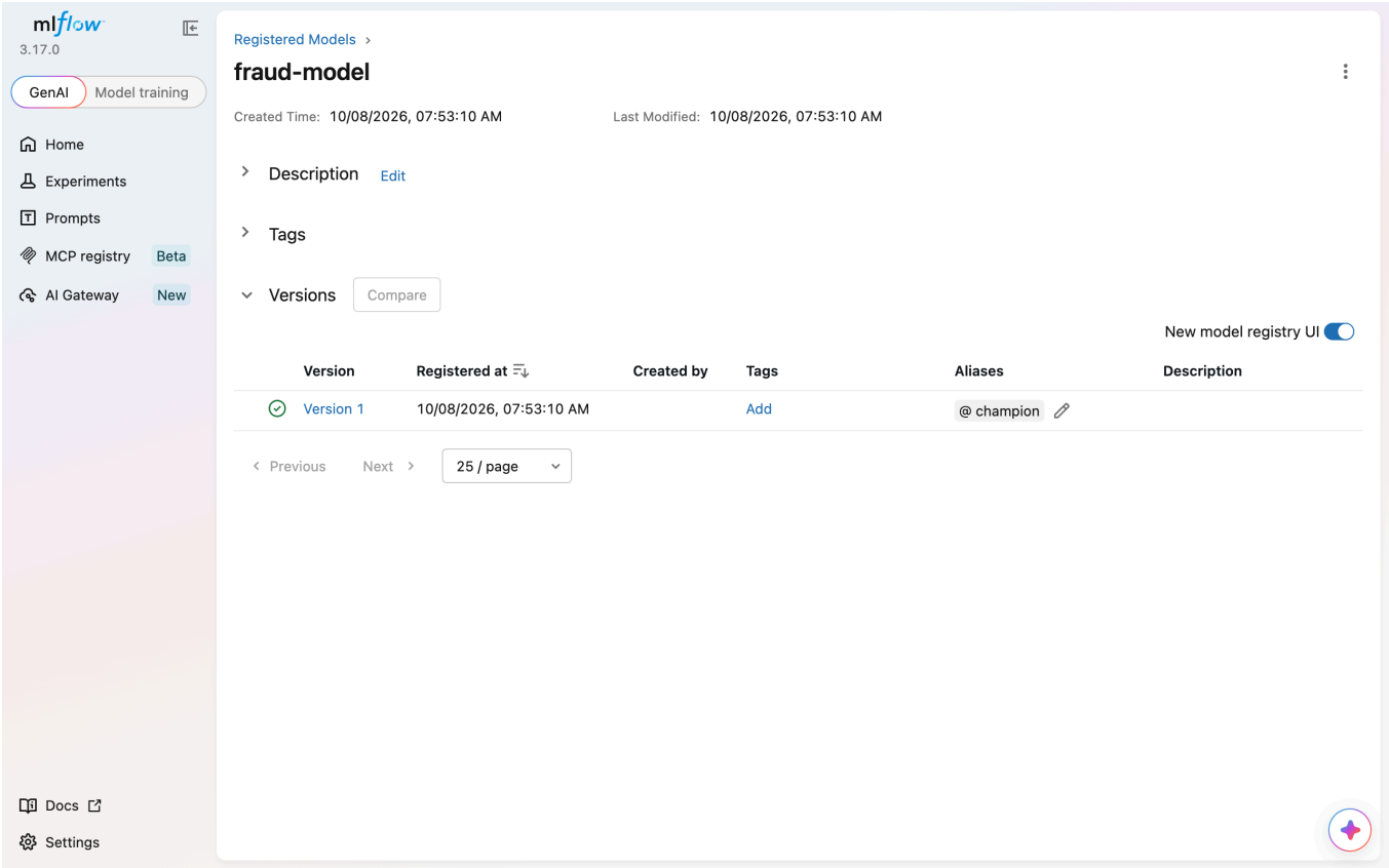
Screenshot 2 - MLflow. MLflow registry page of fraud-model. Version 1 is registered and has the alias champion, which is the only model the service loads.
