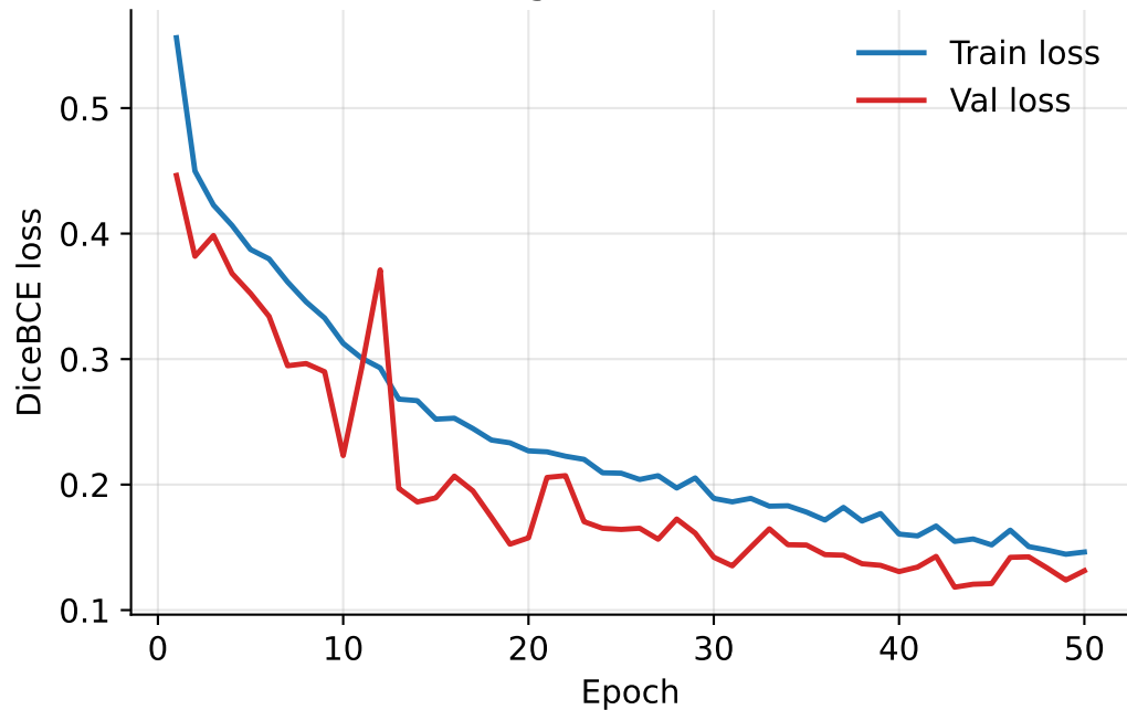
(a) Training and validation loss
