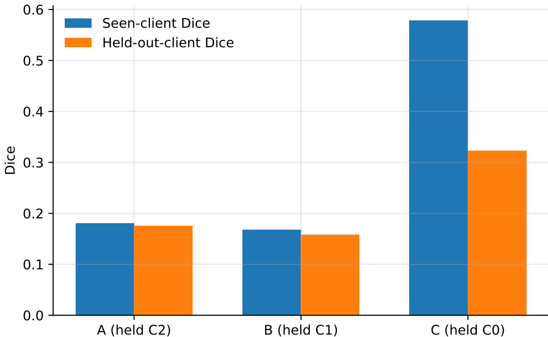
E12 -- Leave-One-Client-Out Generalization
