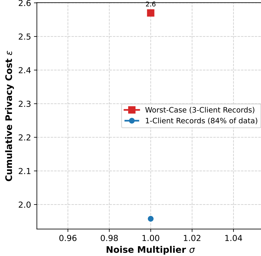
Privacy Budget vs Noise Multiplier \sigma
