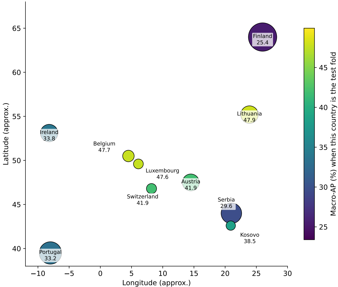
Leave-country-out macro-AP by held-out country BR-LogisticRegression, S4 regime (bubble size = country's patch count)
