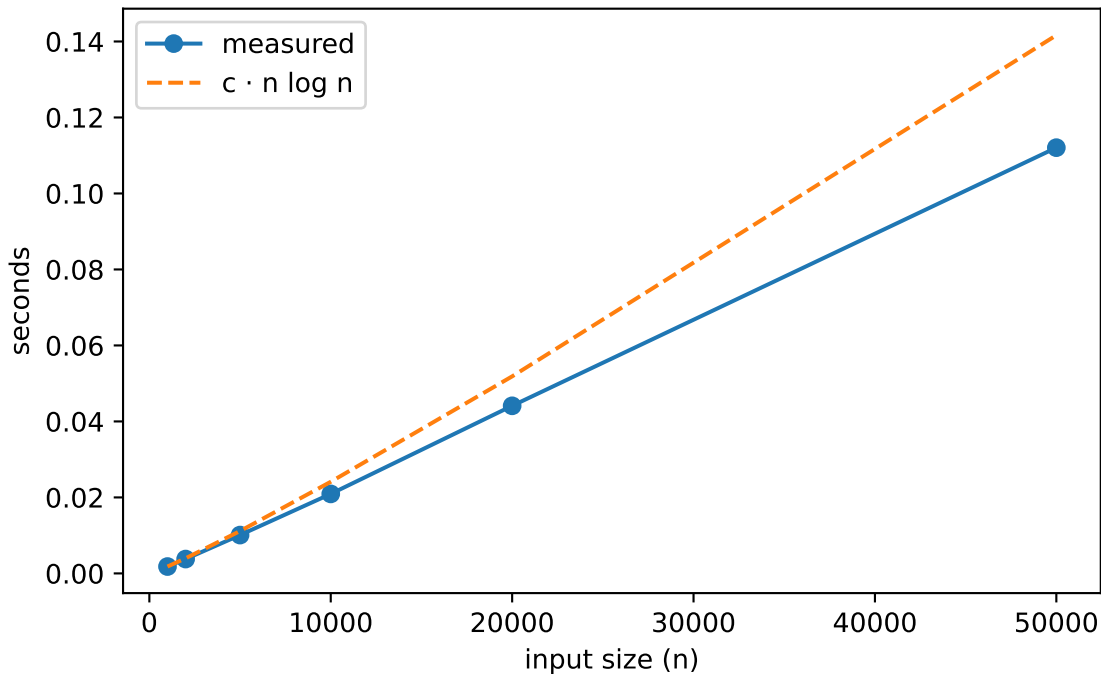
Divide-and-Conquer runtime (expected O(n \log n) )
