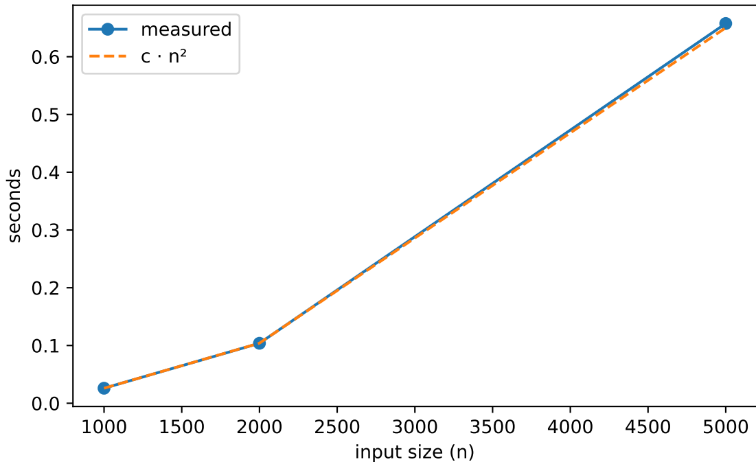
Naive algorithm runtime (expected O(n^2) )
