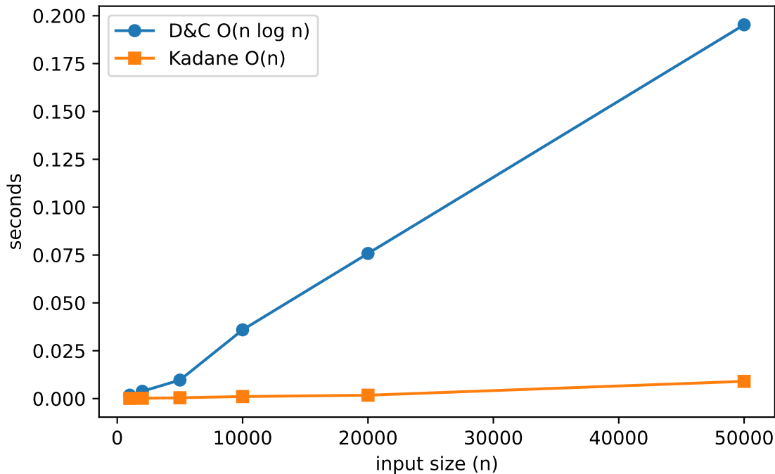
Algorithm Comparison
