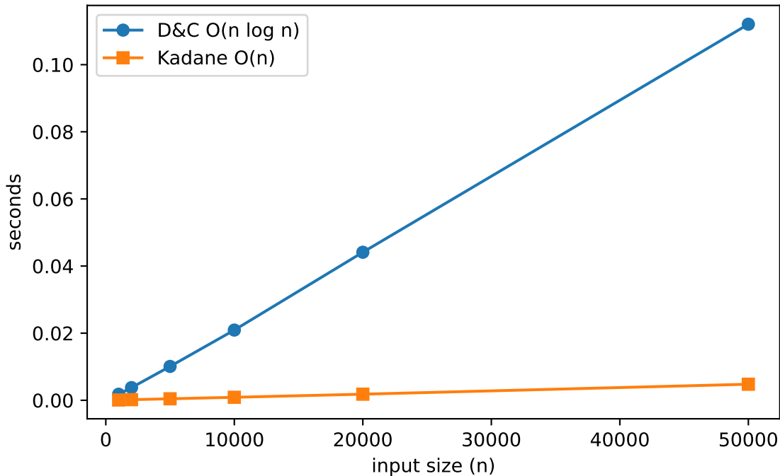
Algorithm Comparison
