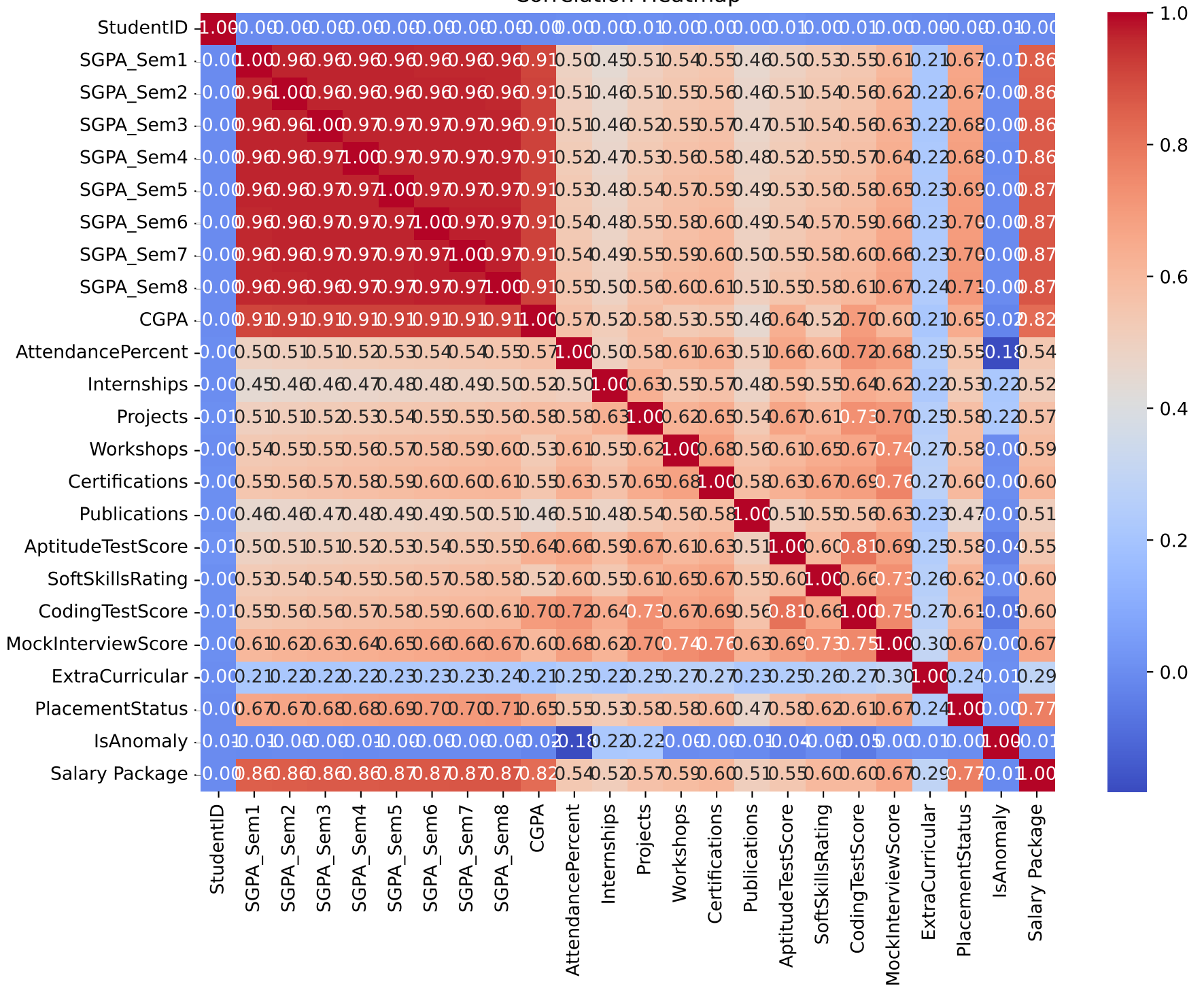
Correlation Heatmap
