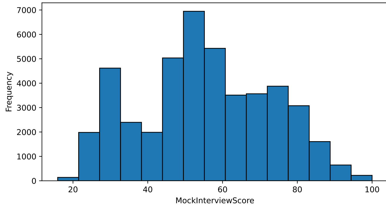
MockInterviewScore
