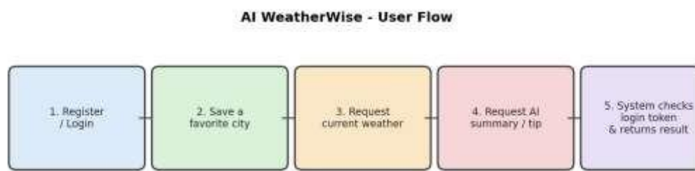
Figure 3: User Flow
