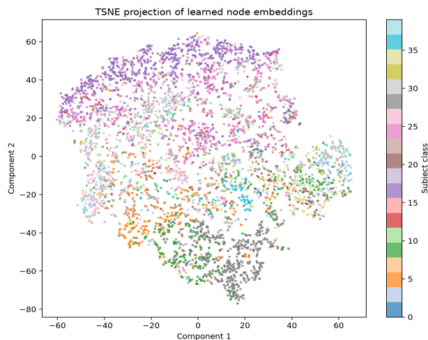
Figure 4(b): Non-linear t-SNE 2D manifold revealing fine-grained semantic sub-communities.
