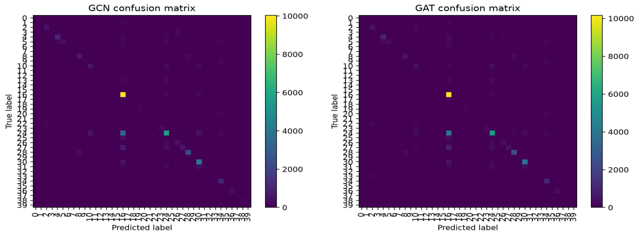
Figure 3(a): GCN 40-class confusion matrix.
