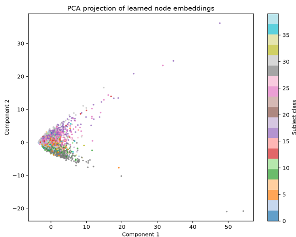
Figure 4(a): Linear PCA 2D projection showing macroscopic domain clusters.
