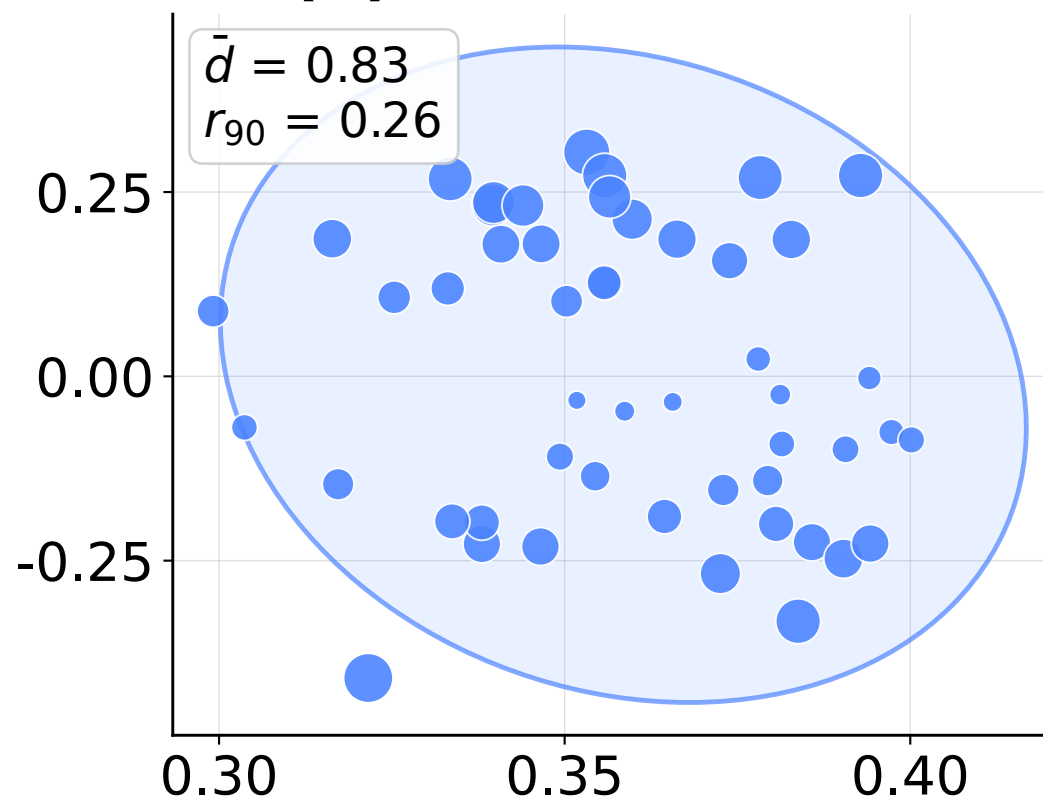
(e) Chatbot-Medical
