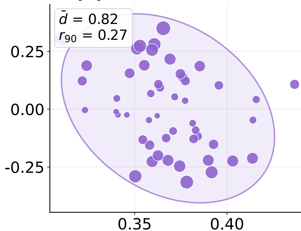
(e) Chatbot-Medical
