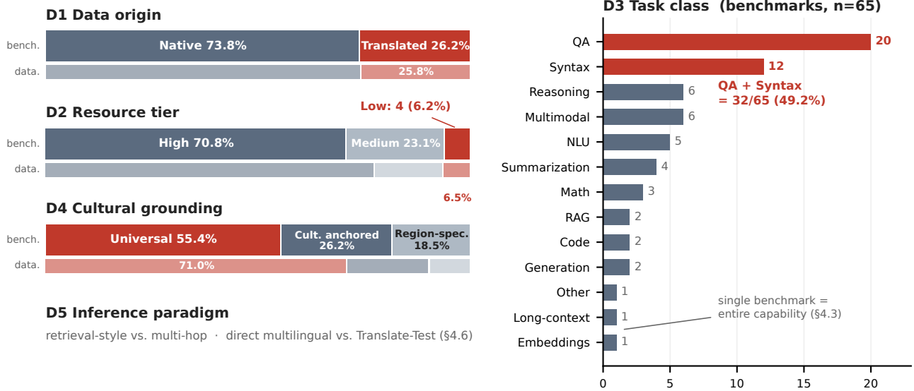
Figure 1: The five-dimensional taxonomy applied to the corpus (thick bars: 65 evaluation benchmarks; thin bars: 31 training datasets). Highlighted segments mark the measured imbalances: 26.2% of benchmarks are built on translated data (D1); only 4 of 65 (6.2%) center low-resource languages (D2); QA and syntax absorb 49.2% of all benchmarks, while long-context, embeddings, and open-ended generation are each represented by one or two benchmarks (D3); and 55.4% are culturally non-specific (D4). The training-data supply mirrors every benchmark-side skew (25.8% translated, 6.5% low-resource, 71.0% universal). D5 (inference paradigm) is analyzed in §4.6.
