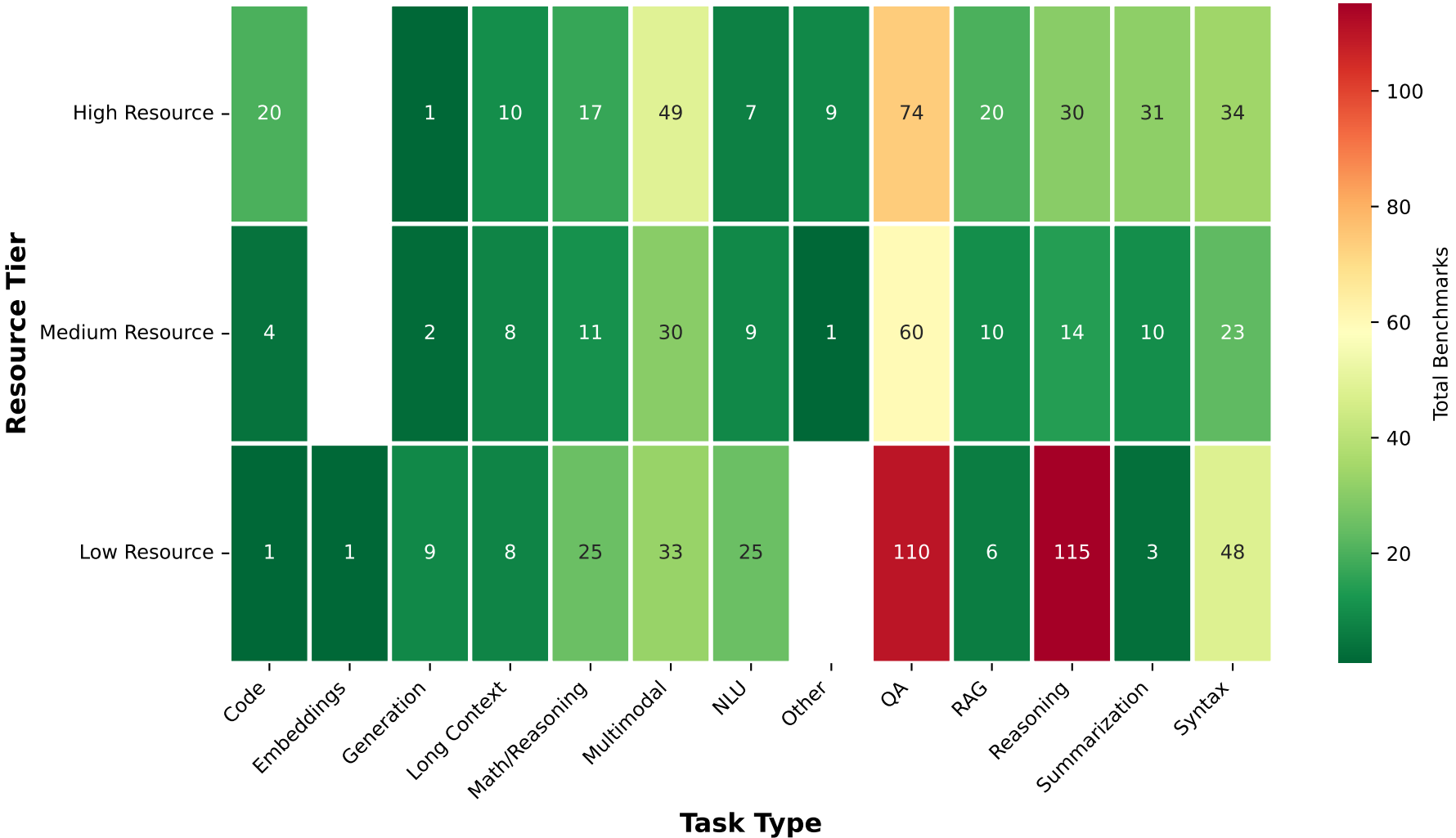
Benchmark Distribution by Linguistic Resource Tier
