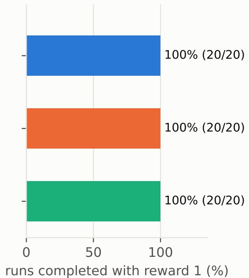
Task success
