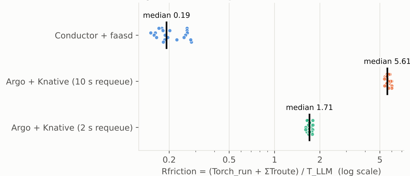
System friction per run
