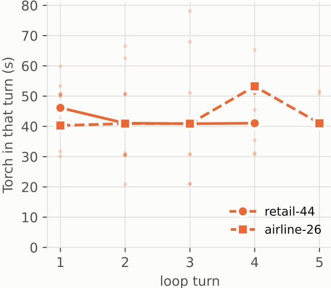
Argo + Knative
