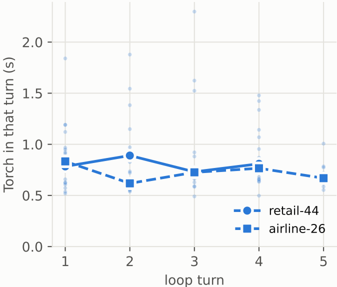
Conductor + faasd
