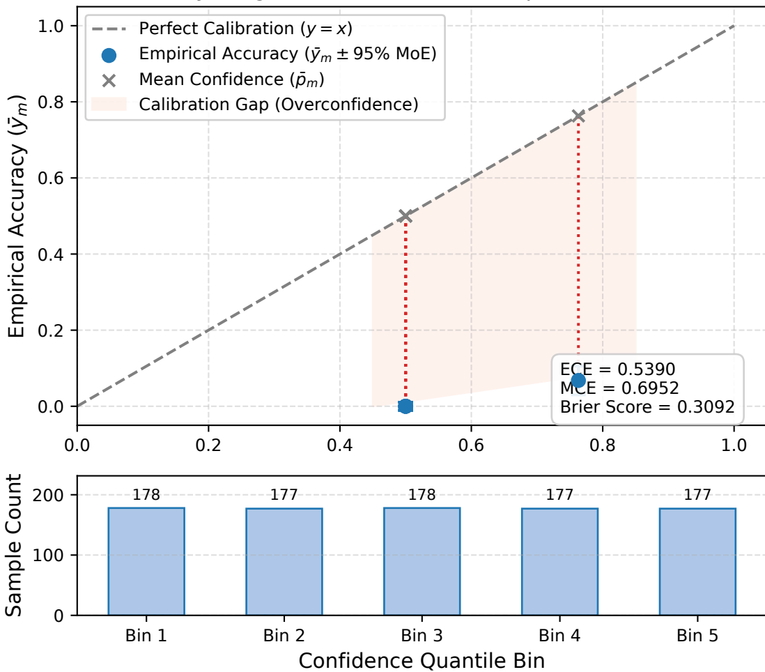
Reliability Diagram (Task 2 GDPR Compliance Predictions)
