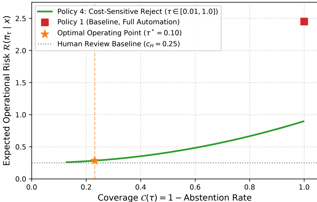
Risk-Coverage Trade-off Curve Across Reject Thresholds \tau
