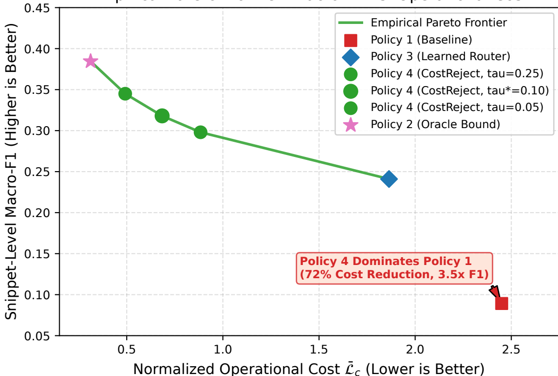
Empirical Pareto Frontier: Macro-F1 vs. Operational Cost
