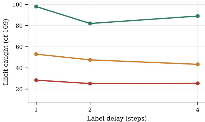
Label accuracy matters more than label speed Bulk feedback Alert-only (AEGIS-CG)
