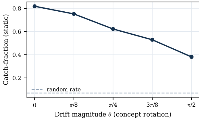
Collapse scales with drift
