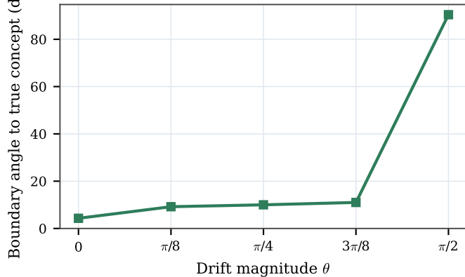
Geometry confirms the cliff
