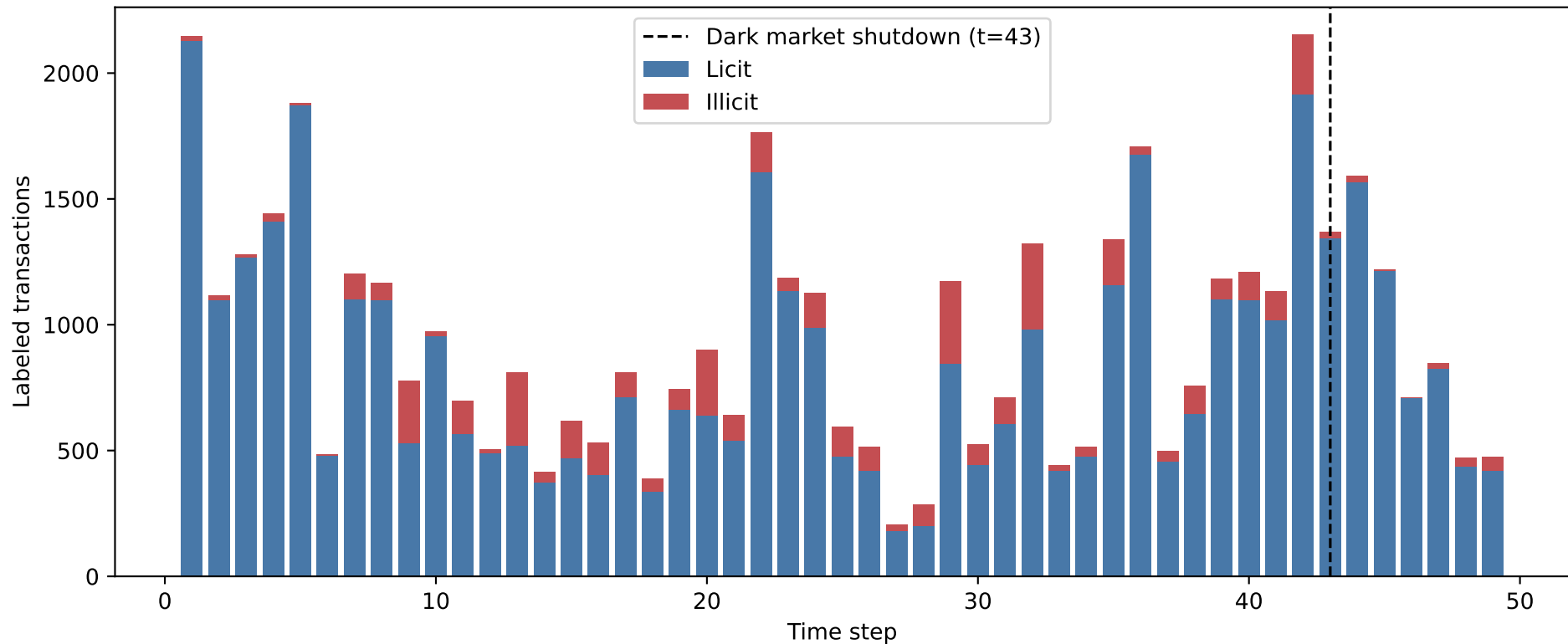
Elliptic: labeled class distribution over time
