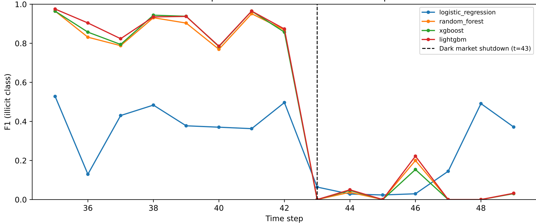
Baseline performance over time: the drift collapse
