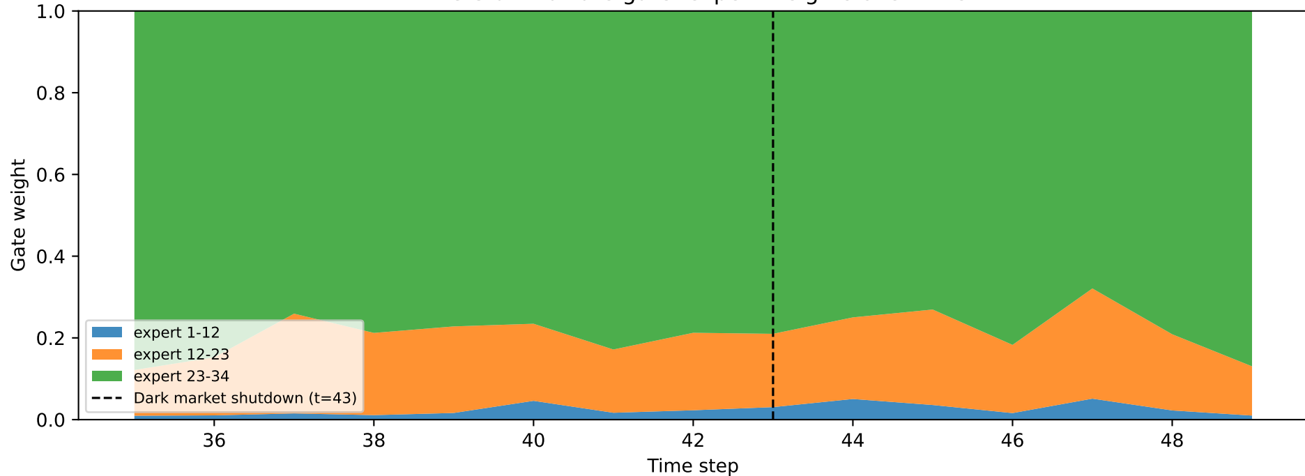
AEGIS drift-aware gate: expert weights over time
