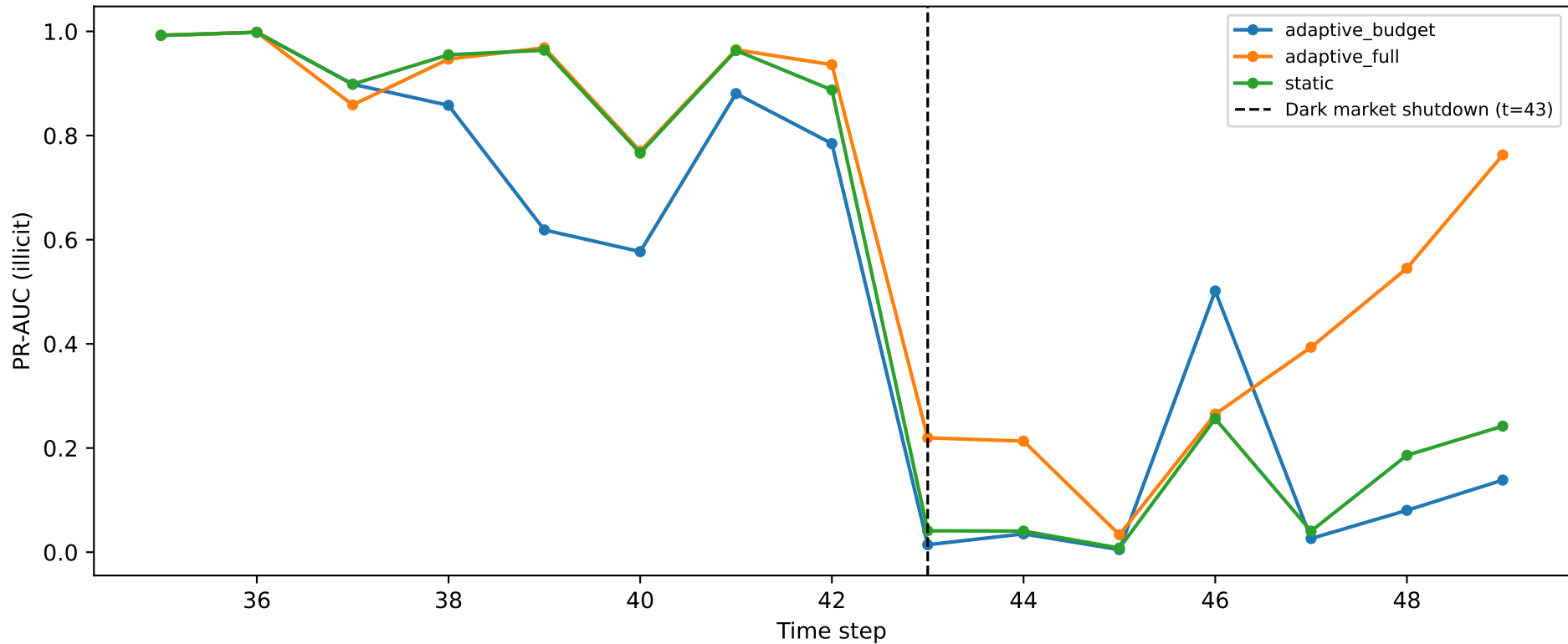
AEGIS detect-and-adapt vs static deployment (budget k=50/\text{step} , delay=1)
