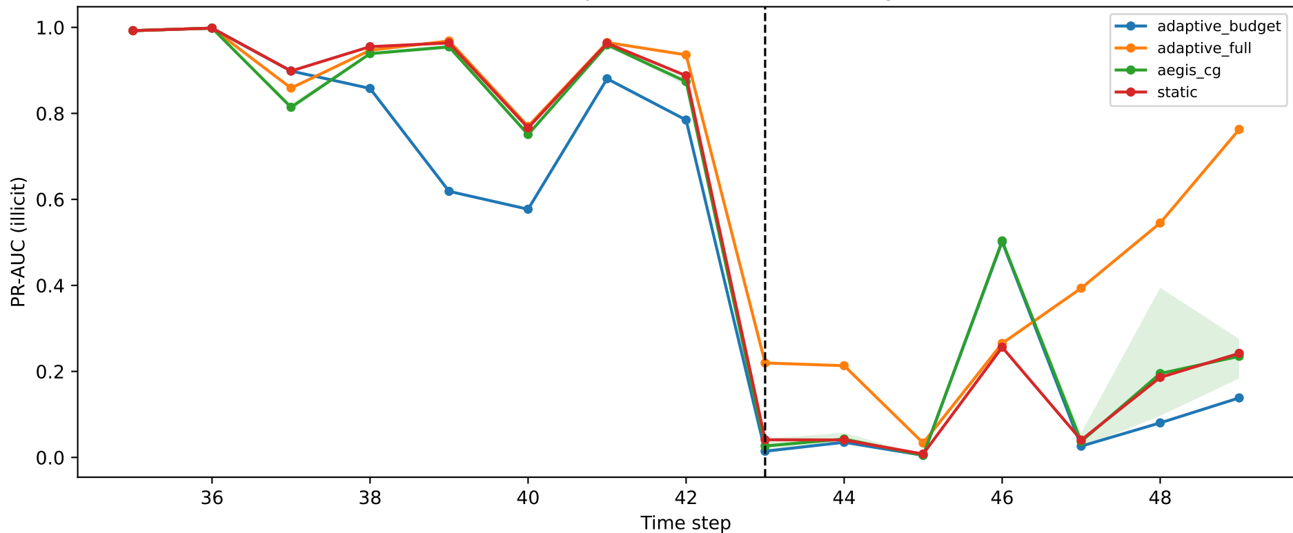
Static vs detect-and-adapt under three feedback regimes (5 seeds)
