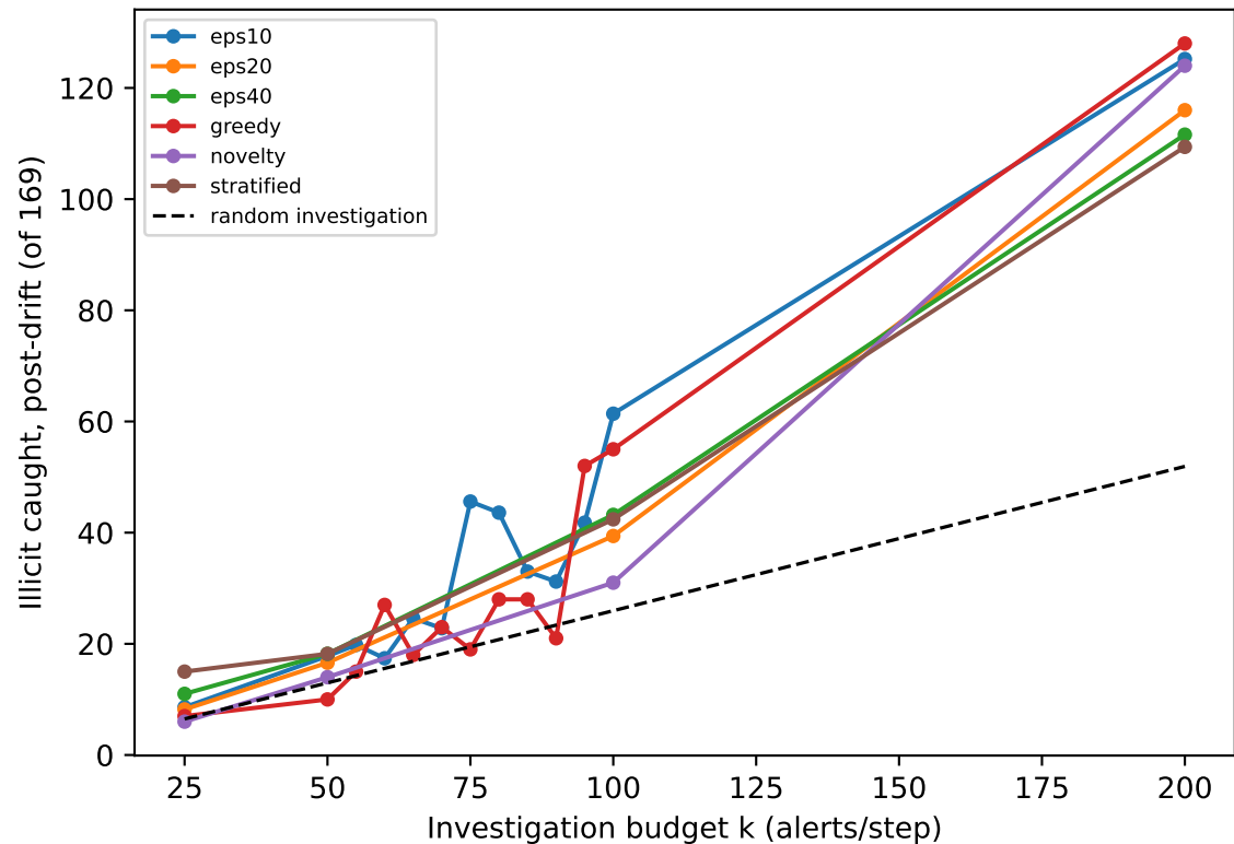
Label-acquisition frontier
