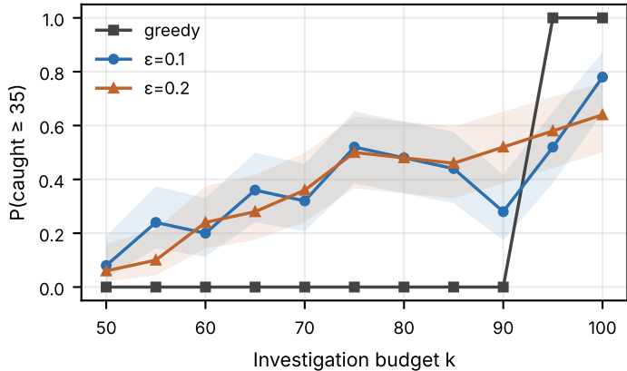
Paper protocol, 50 seeds
