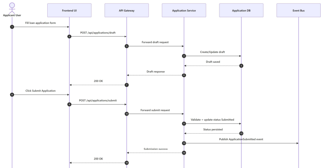
Figure 2 – Loan Application Submission Flow
