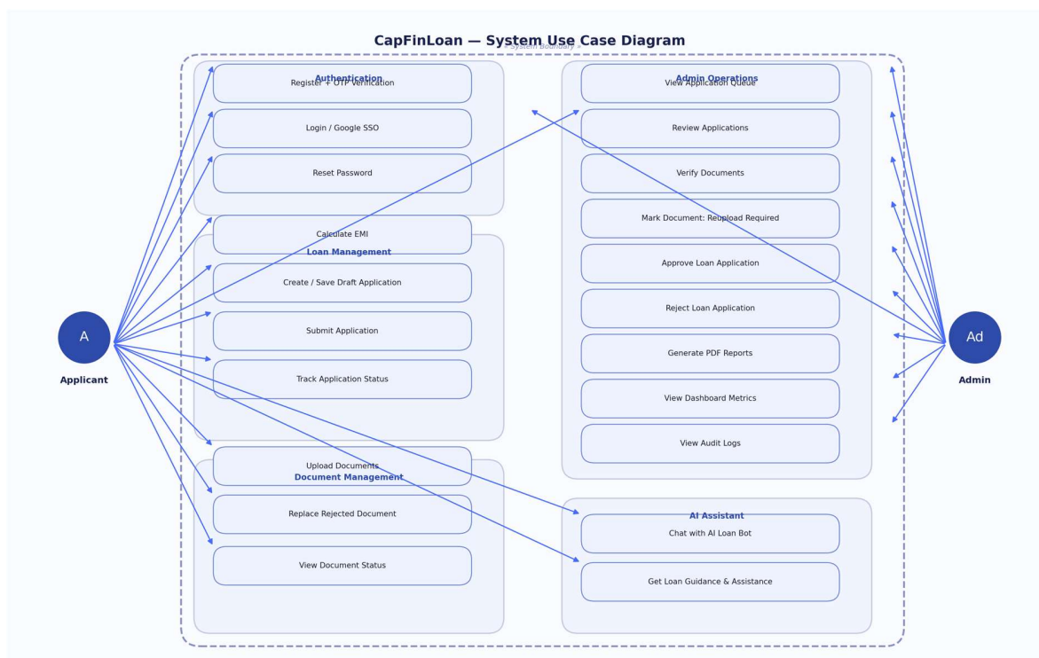
Figure 1 – CapFinLoan System Use Case Diagram
