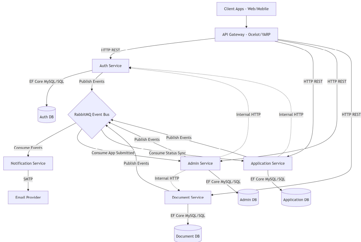
Figure 3 – CapFinLoan Microservices Architecture
