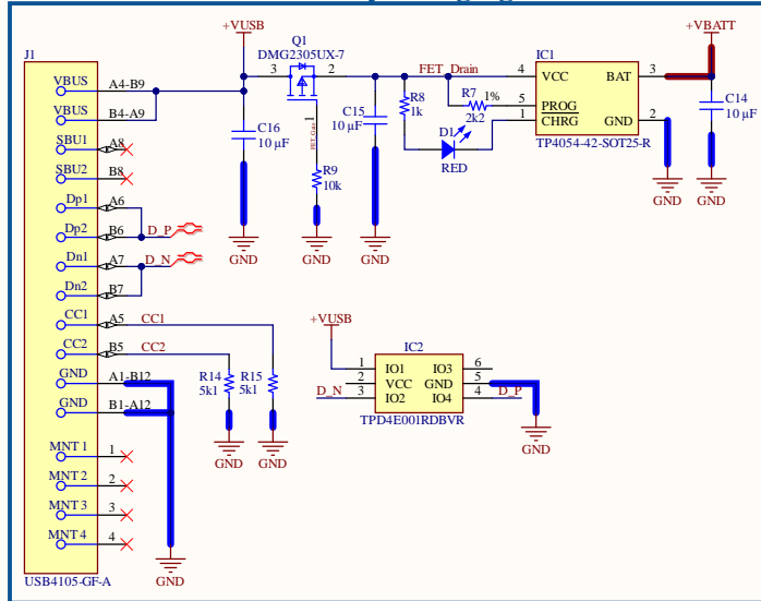
USB-C + Battery Charging Circuit
