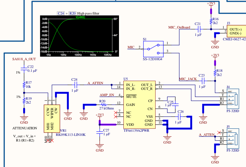
Headphone PA + MIC
