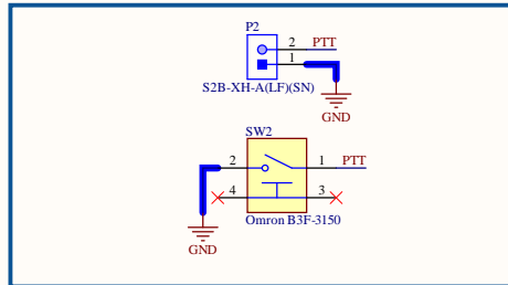
Push To Talk Tactile + Connector
