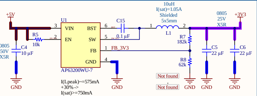
3.3V Buck Converter
