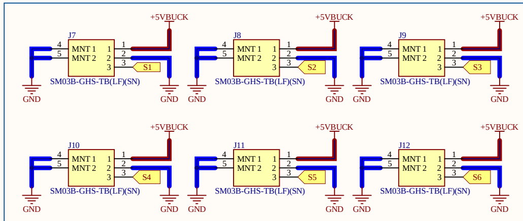
Servo headers
