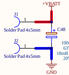
Direct battery voltage(2-6S)
