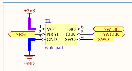
SWD header
