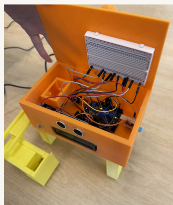
THE ELECTRONICS
