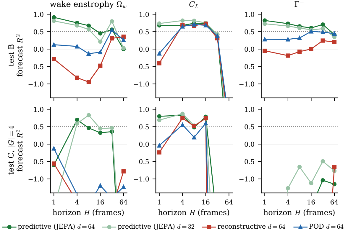
Figure 6: Held-out forecast closure ( R^2 of the Markov rollout) versus horizon H for the wake-enstrophy, C_L , and negative-circulation observables, on the in-distribution test_b (top) and the |G| = 4 extrapolation test_c (bottom), for the predictive latent at d = 64 and d = 32 , the reconstructive autoencoder, and POD. The dotted line marks R^2 = 0.5 . The predictive latent holds wake-enstrophy above the floor to H = 16 ; the reconstructive and linear latents are already below it at H = 1 .
