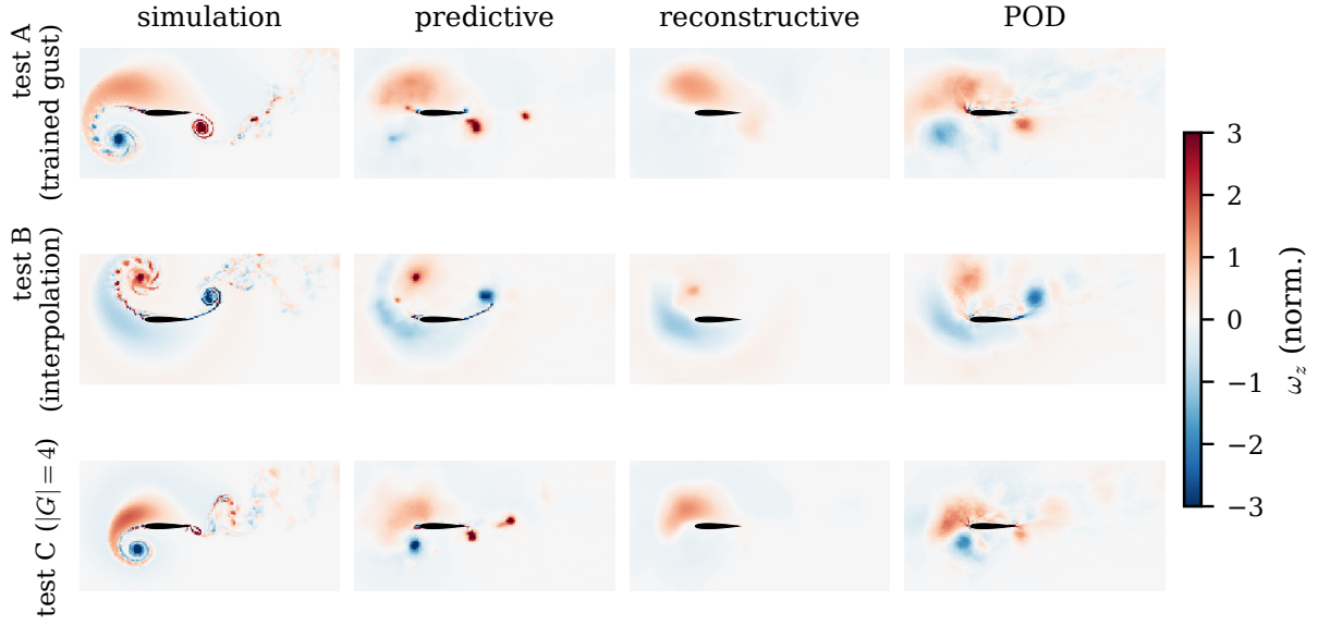
Figure 10: Decoded vorticity at the impact frame on held-out encounters from the three splits (rows: a trained-gust test_a encounter, an interpolation test_b encounter, and a |G|=4 test_c encounter) for the simulation and the predictive, reconstructive, and POD decodes (columns). The predictive decoder is blurry by design but localises the impingement; the reconstructive autoencoder collapses toward a near-uniform field on the held-out interpolation condition, while the linear basis is amplitude-accurate. All families degrade in the |G|=4 regime, reported as the observability boundary of §2.1 rather than as a generalisation claim. Field-space similarity is reframed by the optimal-transport metric of §4.6.
