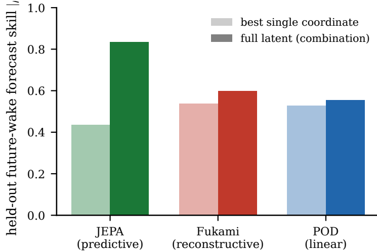
Figure 14: The predictive objective builds a collective wake-forecast code that the reconstructive and linear objectives do not. For each encoder family at matched d = 64 , the held-out forecast skill of the future wake enstrophy \Omega_w(t+H) at H = 16 from the best single latent coordinate (light) and from the full latent combination (dark), on test_b. The predictive (JEPA) latent shows a large gap (combination 0.83, best single 0.44): the wake forecast is distributed across many coordinates. The reconstructive (Fukami) and linear (POD) latents show a near-zero gap and lower skill, so their wake forecast is no better than a single coordinate. Observational probes on the frozen encoders.
