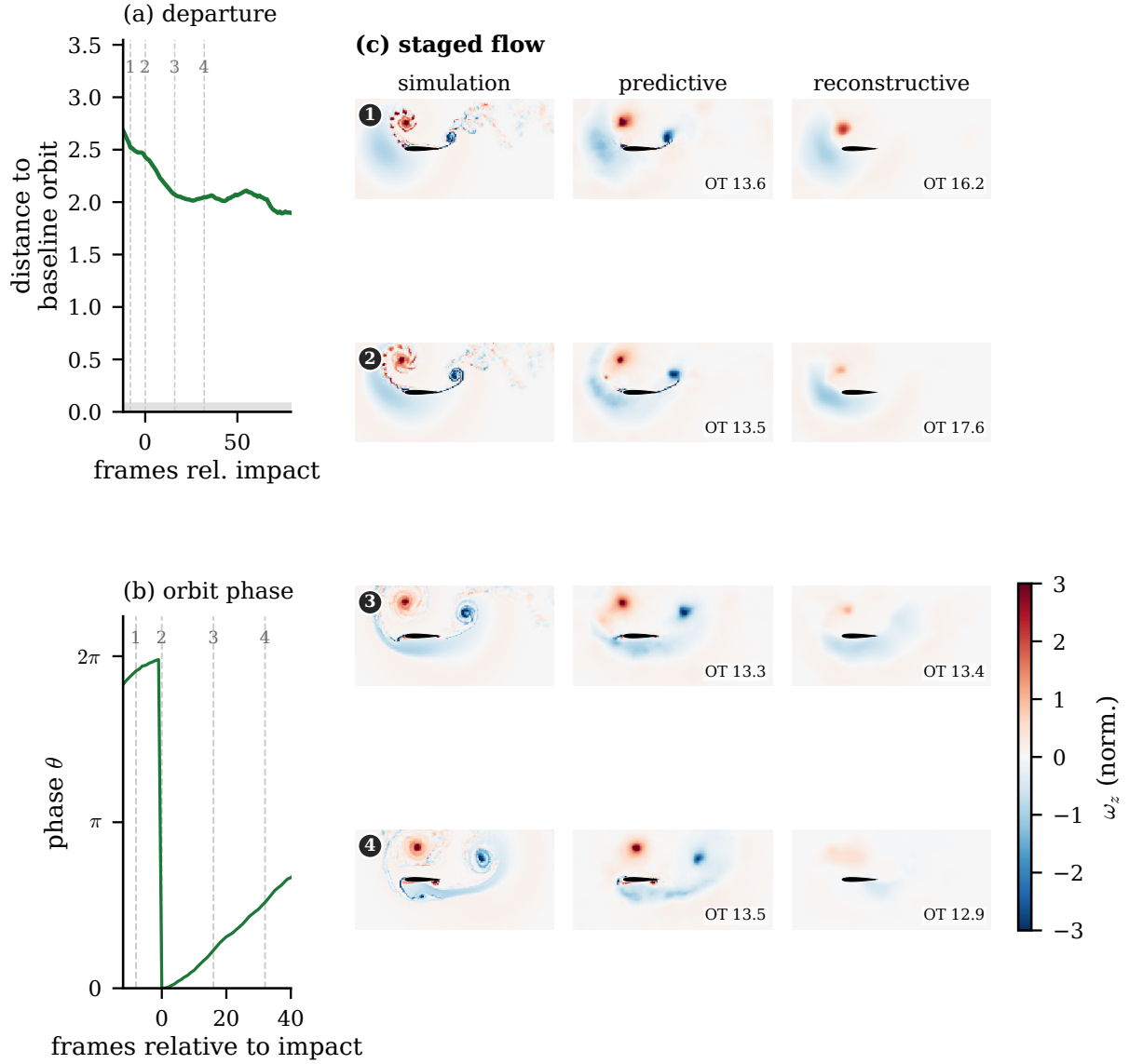
Figure 8: The gust encounter in the predictive latent, for a strong negative gust (G, D, Y) = (-3.0, 1.5, -0.1) . (a) Distance of the gust trajectory to the baseline orbit (full latent, in units of the orbit diameter; the grey band is the baseline orbit thickness): the encounter departs the baseline cycle and only partially relaxes back, without closing within the inter-gust window (§4.5); the single-cycle topology of the encoded latent is established coordinate-free in Figure 7. (b) The orbit phase relative to the impact frame. (c) Mid-plane vorticity at the four stages (rows) for the simulation, the predictive decode, and the reconstructive decode (columns); the predictive decode localises the impingement while the reconstructive decode collapses, with the optimal-transport field distance between each decode and the simulation annotated at each stage (largest for the reconstructive decode near impact). The numbered stages are those of Figure 5.
