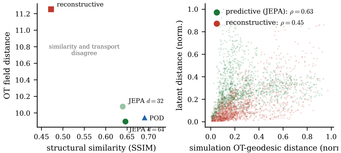
Figure 11: Optimal-transport reconstruction comparison (Tran et al., JFM 2026) on test_b. Unbalanced OT field distance by family at the impact frame, with the structural-similarity ranking shown alongside; the linear basis has the highest similarity but no transport advantage over the predictive decode, while the collapsed reconstructive field is correctly penalised. The Shepard panel shows the per-encounter alignment of latent distance with the simulation OT-geodesic, predictive versus reconstructive.
