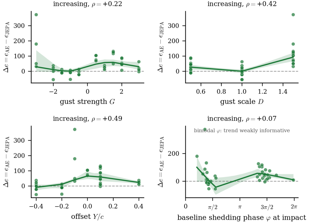
Figure 9: Per-encounter paired improvement \Delta e = e_{\text{AE}} - e_{\text{JEPA}} in held-out wake-enstrophy error against the gust strength G , core diameter D , wall-normal offset Y , and the baseline shedding phase at impact \phi (test_b, n = 42 ); positive \Delta e means the predictive latent carries the smaller error. Each panel shows the per-encounter values, a locally weighted (LOWESS) trend, and a bootstrap band over encounters. The predictive advantage grows with D and toward off-midplane Y ; the shedding-phase axis falls into two clusters because impact is fixed near a single convective instant.
