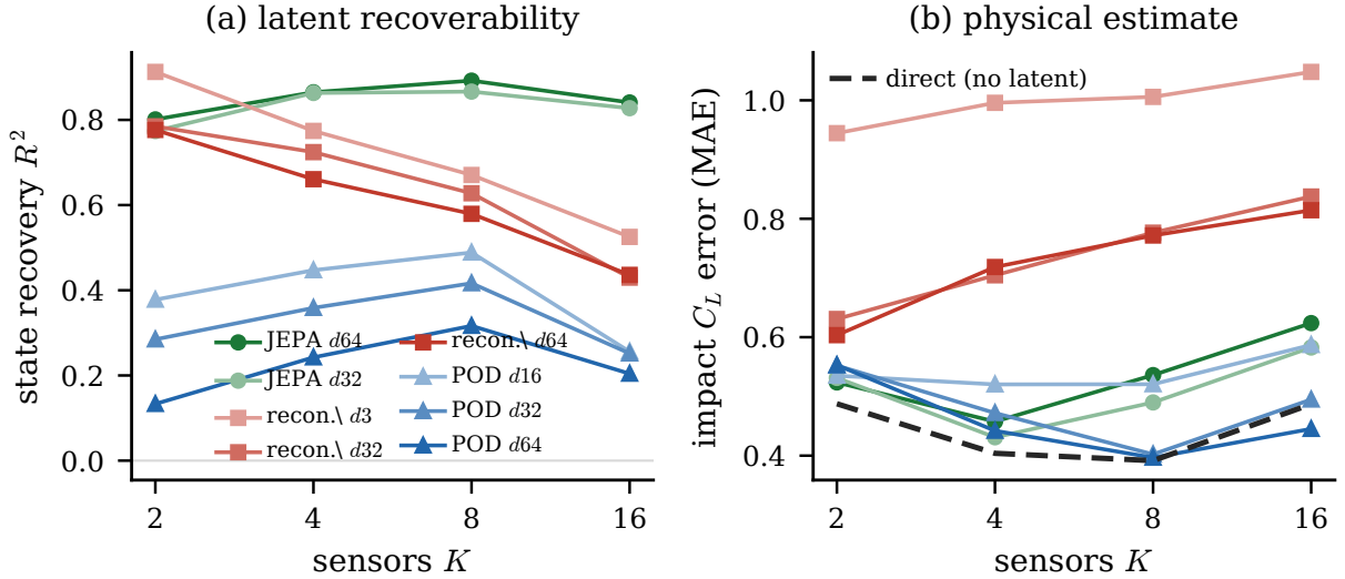
Figure 13: Cross-family pressure observability under the target-conditioned (TCSI) sensor placement. (a) Latent-state recovery R^2 versus sensor count K : the predictive (JEPA) state is the most recoverable at K \geq 4 , the linear basis the least. (b) The physical estimate, impact C_L mean absolute error routed through each family's recovered latent, with the direct pressure-to- C_L baseline (dashed). The reconstructive d = 3 latent is the easiest to recover (highest R^2 at low K ) yet gives the worst lift estimate, and the lift is read most accurately directly from the pressure.
