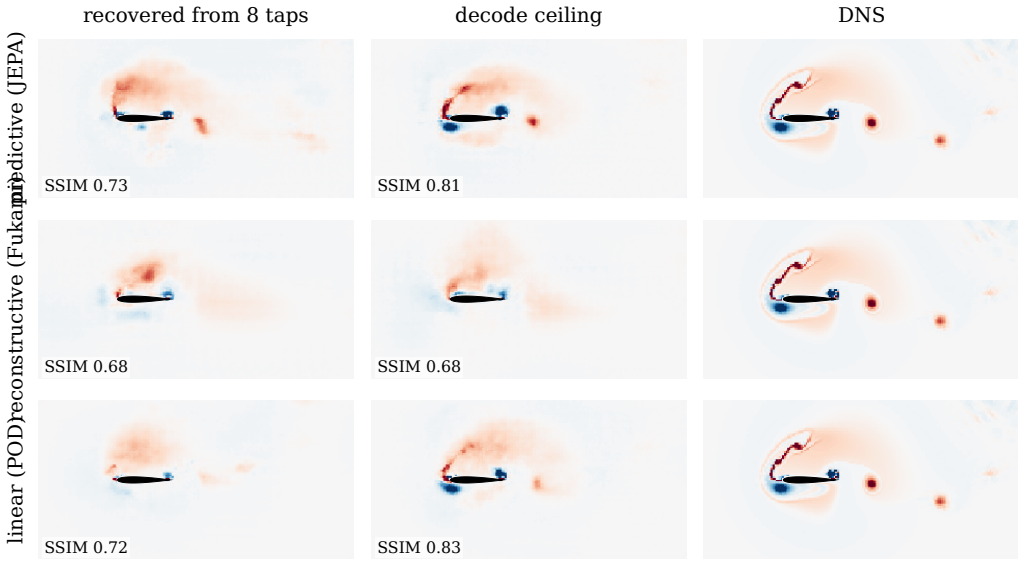
Figure 26. Flow recovered from eight wall-pressure taps on the representative held-out encounter of figure 16, at the impact-side frame, one row per family. Columns: the field decoded from the pressure-recovered coefficient state, the decode ceiling (the same decoder applied to the encoded state, no pressure step), and the simulation; per-panel structural similarity annotated. The comparison is within each row, since the decoders' ceilings differ (§5.3); the ceiling-to-recovered gap is the cost of the pressure step.
