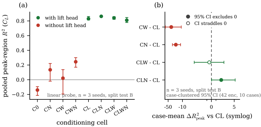
Figure 23. Paired peak-region lift R^2 per conditioning-cube cell (left) and case-mean deltas against the lift-only cell CL (right, symmetric-log axis, 95 % case-clustered bootstrap intervals over the 42 in-distribution test encounters of 10 cases); filled markers mark intervals that exclude zero. The near-body lift-focused predictive state cell (CLN) is the unique positive increment; the no- L cells sit one to two orders of magnitude lower.
