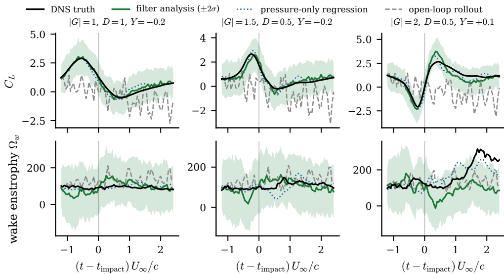
Figure 16. The estimator tracks the encounter from wall pressure alone. Columns are representative held-out encounters at |G| = 1, 1.5 and 2 ; rows are the lift coefficient and the wake enstrophy. Each panel shows the DNS truth, the filter analysis with its \pm 2\sigma ensemble band, the pressure-only regression, and the open-loop rollout; the vertical line marks impact. The filter follows the load through impact and relaxation where the open-loop forecast loses it and the pressure-only regression goes stale.
