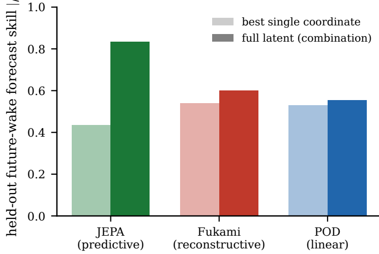
Figure 15: The predictive objective builds a collective wake-forecast code that the reconstructive and linear objectives do not. For each encoder family at matched d = 64 , the held-out forecast skill of the future wake enstrophy \Omega_w(t+H) at H = 16 from the best single latent coordinate (light) and from the full latent combination (dark), on test_b. The predictive (JEPA) latent shows a large gap (combination 0.83, best single 0.44): the wake forecast is distributed across many coordinates. The reconstructive (Fukami) and linear (POD) latents show a near-zero gap and lower skill, so their wake forecast is no better than a single coordinate. Observational probes on the frozen encoders.
