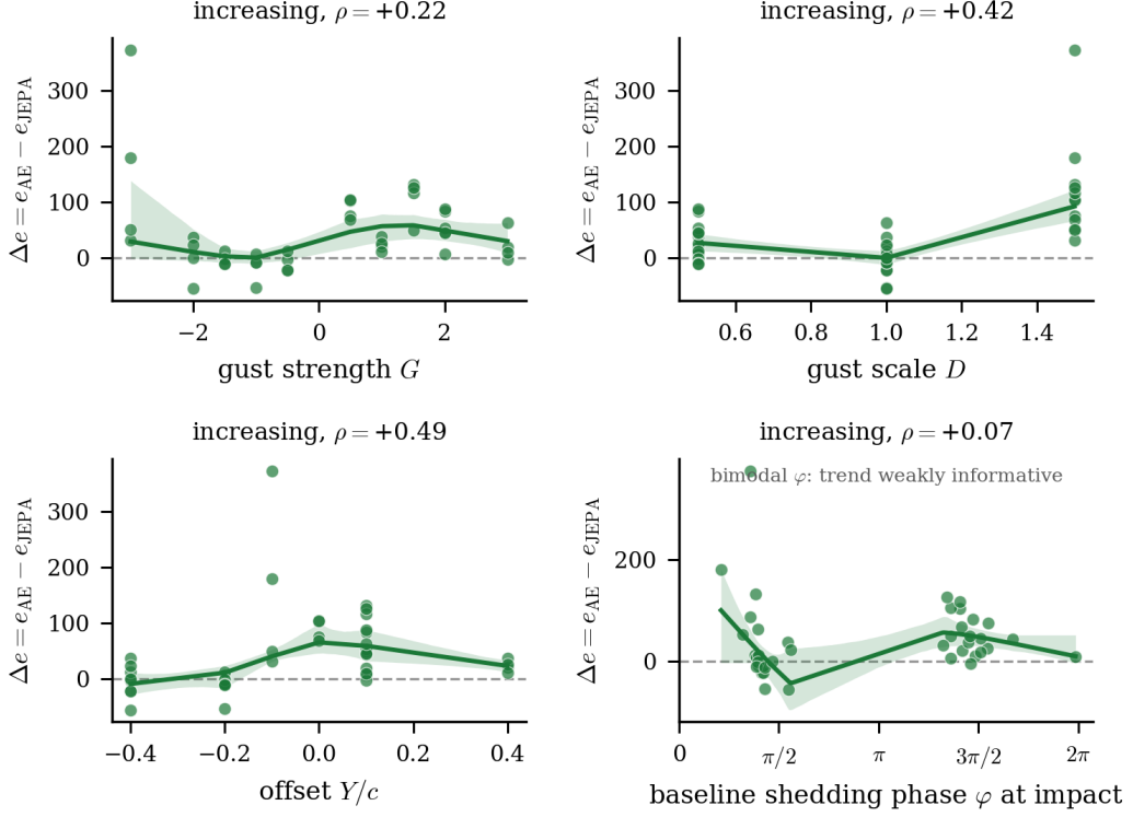
Figure 10: Per-encounter paired improvement \Delta e = e_{\text{AE}} - e_{\text{JEPA}} in held-out wake-enstrophy error against the gust strength G , core diameter D , wall-normal offset Y , and the baseline shedding phase at impact \phi (test_b, n = 42 ); positive \Delta e means the predictive latent carries the smaller error. Each panel shows the per-encounter values, a locally weighted (LOWESS) trend, and a bootstrap band over encounters. The predictive advantage grows with D and toward off-midplane Y ; the shedding-phase axis falls into two clusters because impact is fixed near a single convective instant.
