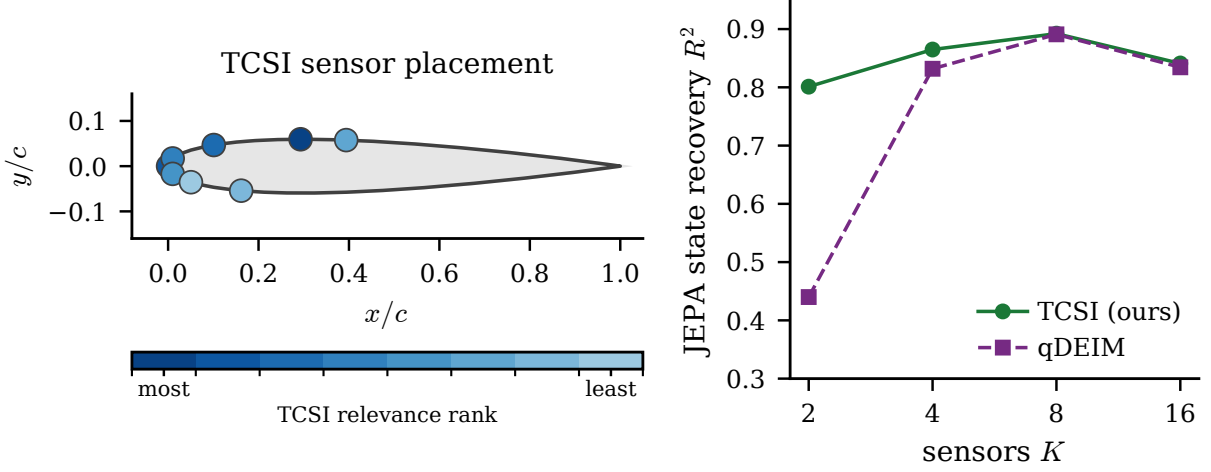
Figure 17: Sparse-sensor placement. (a) The target-conditioned (TCSI) taps on the NACA 0012 surface, a single ranked set with one marker per tap coloured from dark (picked first, most informative) to light (least); the greedy picks are nested, so the two darkest are the decisive K = 2 pair and the eight shown are the K = 8 set. They cluster near the leading edge, where the gust impinges. (b) Predictive-state recovery (held-out test R^2 ) versus sensor count for the target-aware selection (TCSI) and the target-blind QR-pivot optimum of the pressure modes (qDEIM): the target-aware placement helps at K = 2 but the two converge by K \geq 4 , so the recoverability result is not an artefact of the placement.
