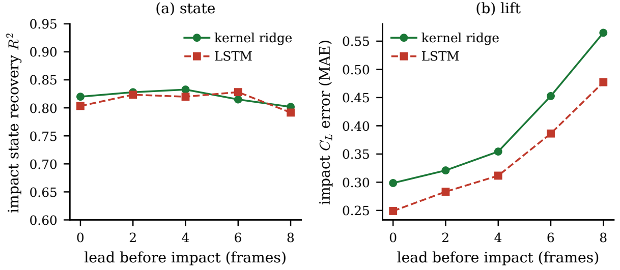
Figure 19: Predicting the impact before it occurs. (a) Impact-state recovery R^2 and (b) impact-lift C_L mean absolute error versus the lead, the number of frames before impact at which the pre-impact pressure window ends, for the kernel-ridge and LSTM estimators ( K = 8 TCSI taps, test_b). The impact state is recoverable to eight instants ahead; the lift to about four, with the LSTM the more accurate lift estimator at short lead.
