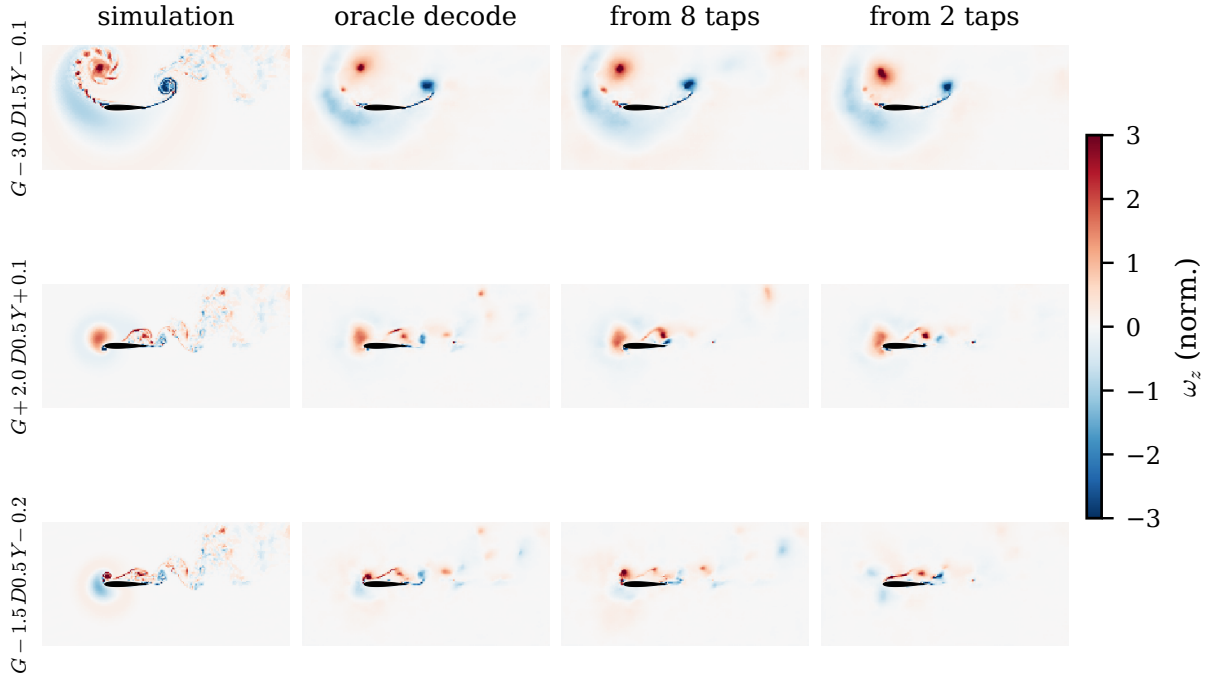
Figure 18: Flow recovered from sparse wall pressure on three held-out encounters (rows, labelled by (G, D, Y) ). Columns: the simulation, the oracle decode (the visualisation decoder applied to the simulation-encoded latent), and the decode of the latent estimated from K = 8 and K = 2 TCSI pressure taps. From eight taps the predictive latent recovers the leading-edge vortex and shear layer close to the oracle; two taps capture the gross impingement. The decoder is blurry by design (§4.6).
