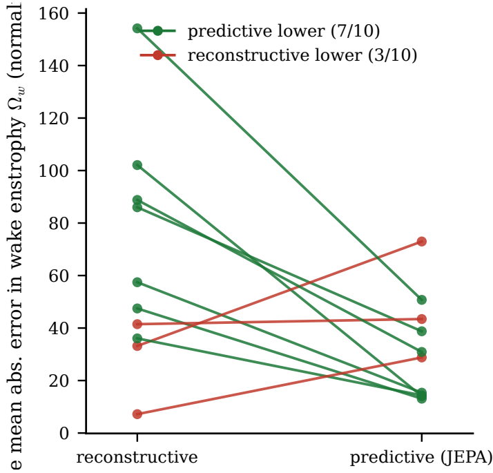
Figure 5. Per-case wake-entrstrophy closure, the honest case-level view of the headline result. Each line is one held-out test_b case (ten in all), connecting the reconstructive autoencoder's per-case mean absolute error (left) to the predictive latent's (right) at H = 16 ; a downward line favours the predictive latent. The predictive latent gives the lower error on seven of the ten cases (median per-case improvement positive, case-level signed-rank significant), with three cases favouring the reconstructive baseline: the advantage is real at the case level but not uniform, which is why the case-level multiplicity correction is not passed and the claim is stated at encounter level with this spread shown.
