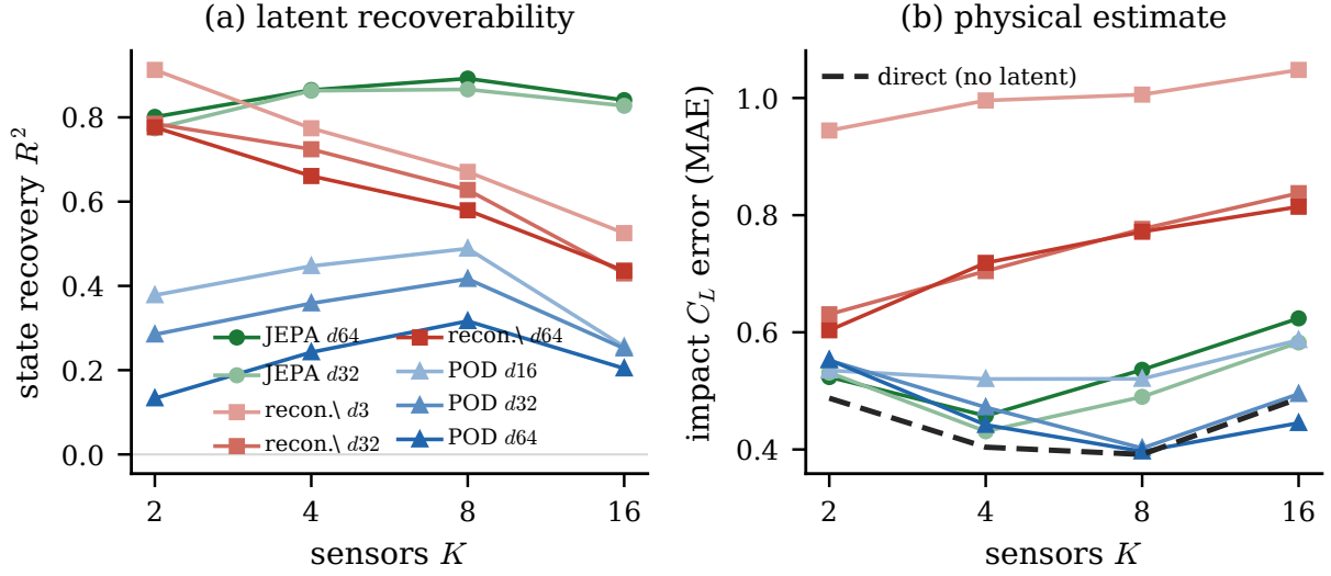
Figure 13: Cross-family pressure observability on v2 under the TCSI placement. (a) Latent-state recovery R^2 versus sensor count: the predictive (JEPA) state is the most recoverable at K \geq 4 , POD the least. (b) The physical estimate, impact C_L mean absolute error routed through each family’s recovered latent, with the direct pressure-to- C_L baseline (dashed). The contrast is the point: the reconstructive d = 3 latent is the easiest to recover (highest R^2 at low K ) yet gives the worst lift estimate, and the lift is read most accurately directly from the pressure.
