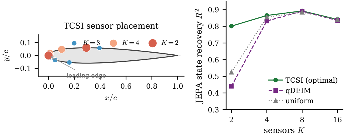
Figure 12: Sparse-sensor placement on v2. (a) The target-conditioned (TCSI) taps for K=2, 4, 8 on the NACA 0012 surface; they cluster near the leading edge on both surfaces. (b) Predictive-state recovery (held-out test_b R^2 ) versus sensor count for TCSI, qDEIM, and uniform placement: optimal placement is decisive at K=2 and the methods converge by K \geq 4 .
