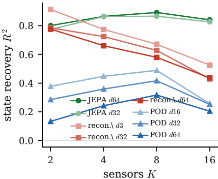
(a) latent recoverability
