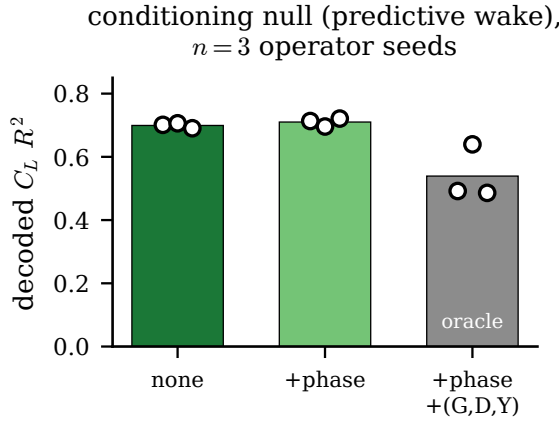
Figure 19. The conditioning null on the shared direct multi-horizon forecaster (demoted from the forecast figure 8): decoded lift R^2 of the tuned forecaster on the wake-supervised predictive state latents under no covariate, an added phase covariate, and an added ( G , D , Y ) gust-parameter oracle (three operator seeds per arm). The deployable phase covariate is a wash with the unconditioned forecaster, while the gust-parameter oracle degrades it.
