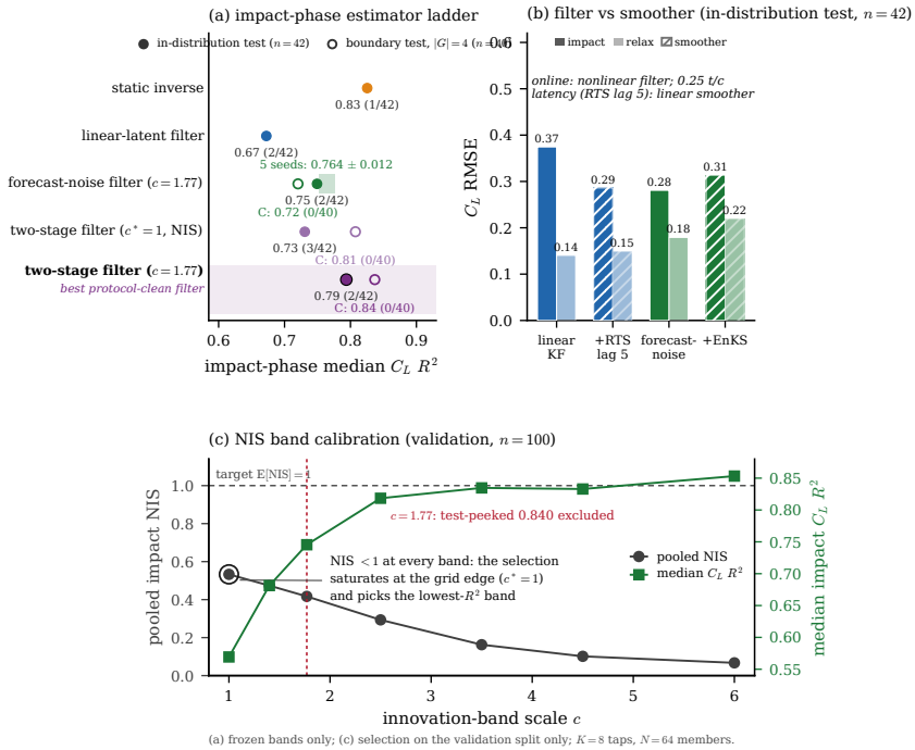
Figure 30. Estimator calibration and selection (in-distribution test, validation and, through the open markers, boundary test sets; parentetical counts on the ladder are large-error encounters, impact-phase R^2 < -1 , per set). (a) The impact-phase estimator ladder with the five-seed member-noise band, open markers the frozen boundary test values; (b) the filter against the fixed-lag smoother; (c) the band-scale calibration on the held-out training encounters, where innovation consistency and tracking disagree and the selection saturates at the grid edge.
