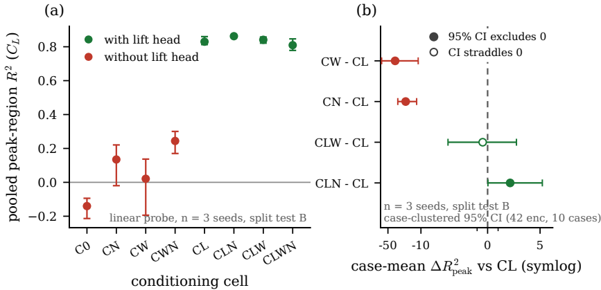
Figure 16. Paired peak-region lift R^2 per conditioning-cube cell (left) and case-mean deltas against the lift-only cell CL (right, symmetric-log axis, 95 % case-clustered bootstrap intervals over the 42 in-distribution test encounters of 10 cases); filled markers mark intervals that exclude zero. The near-body lift-focused predictive state cell (CLN) is the unique positive increment; the no- L cells sit one to two orders of magnitude lower.
