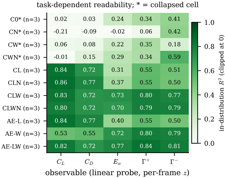
Figure 18. Task-dependent readability (in-distribution test set, linear probes on the per-frame state, seed mean over three encoder seeds per cell): lift and drag follow the L head, the wake block ( E_w , \Gamma^\pm ) follows the W head or the reconstruction objective, and collapsed cells (asterisks) read nothing linearly.
