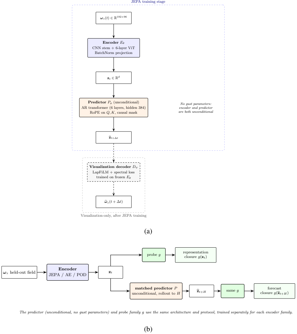
Figure 3. The predictive model and how it is evaluated. (a) The encoder maps the mid-plane vorticity field to a latent \mathbf{z}_t , and the autoregressive predictor advances the latent from its own history; no gust parameters enter the encoder or the predictor. The two auxiliary observable heads (lift and wake) read \mathbf{z}_t during JEPa training with small weights and are not part of the latent-prediction loss; they are omitted from the schematic for clarity. The visualisation decoder is trained only after the encoder is frozen and is used solely for the diagnostic decodes of §4.6, never in the predictive loss. (b) Evaluation applies the same predictor and probe family g to every encoder family: a probe on the simulation-encoded latent measures representational closure, the headline, and the same probe on the rolled-out latent \hat{\mathbf{z}}_{t+H} measures forecast closure, reported as secondary.
