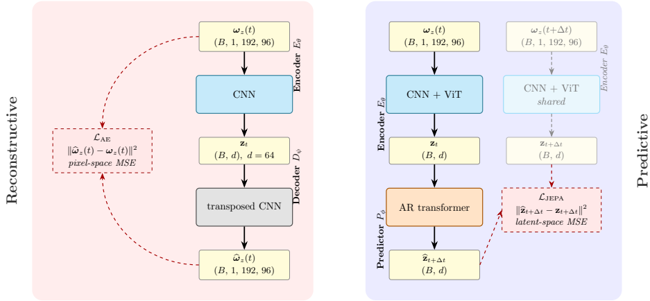
Figure 13. Predictive versus reconstructive training. Left: the reconstructive autoencoder encodes the field at t , decodes it, and incurs a field-space error. Right: the predictive model encodes the fields at t and t + \Delta t with shared weights and incurs a latent-space error between the predicted and observed target embeddings, with no field-space loss and no decoder during training. This is the contrast the matched-predictor protocol of §3.2 evaluates; the visualisation decoder is trained only afterwards, on the frozen encoder.
