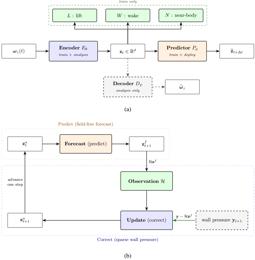
Figure 4. The framework, from representation to deployment. Each module in (a) carries the stages in which it is active: the encoder is used in training and in the analyses that read \mathbf{z}_t , the three supervision heads are dropped once training ends, the predictor is the only trained module that also runs at deployment, and the visualisation decoder is trained on the frozen encoder and serves analysis alone. (a) The encoder maps the mid-plane vorticity field \omega_z \in \mathbb{R}^{192 \times 96} to a latent \mathbf{z}_t through a CNN stem, a six-layer ViT and a BatchNorm projection, and the predictor advances the latent from its own history in either of its two variants: the six-layer autoregressive transformer with rotary temporal positions of table 11, or the direct multi-horizon forecaster of §3.2.1. No gust parameters enter either network; both are unconditional. The heads read \mathbf{z}_t during training under a smooth- L_1 loss at unit weight, mapping it to the scalar lift C_L(t) ( L ), an 80-dimensional wake observable ( W ) and an 80-dimensional Chang lift-element observable ( N ); none is part of the latent-prediction loss. The decoder D_\psi pairs LapFiLM with a spectral loss. (b) At deployment the pressure-only predict-correct estimator advances an ensemble of 64 members field free through the matched forecast model, then corrects them from 8 span-averaged wall-pressure taps held out from training and placed by the per-model sensor selection. The innovation is the measured minus the predicted observation, in tap space for the base filter of §3.3.1 and in encoded latent space for the filters of §3.3.2 and §3.3.3, and the update is a stochastic ensemble Kalman step at inflation \rho = 1 with calibrated \mathbf{Q} and \mathbf{R} . No vorticity field enters the loop, the state is the same 32-vector at every step, and the lift and wake probes never enter the innovation. The evaluation protocol applied identically to every encoder is figure 21 (appendix A).
