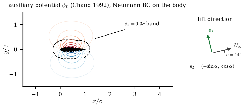
Figure 24. [APA-C10] The Chang auxiliary potential \phi_L of equation (A 1) on the cache grid (contours), the feathered \delta_n = 0.3c supervision band (dashed) and the airfoil footprint; the inset shows the lift direction \mathbf{e}_L against the inclined freestream at \alpha = 14^\circ .
