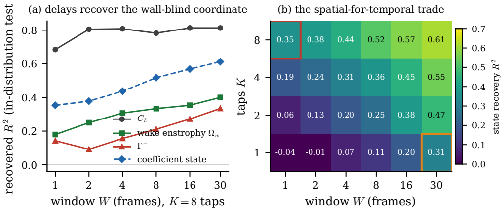
Figure 12. [S4-C3]Sensors traded for delays. (a) Recovery of each observable from eight wall-pressure taps against the length of the pressure window (in-distribution test set); the wall-blind wake circulation rises with the window while the force, visible at one instant, does not. (b) Coefficient-state recovery over the tap-count by window-length grid, with the single-tap, thirty-frame cell and the reference eight-tap, single-frame cell outlined: a long window with few taps matches a short window with many.
