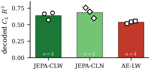
(a) shared REX operator, encoder seeds
