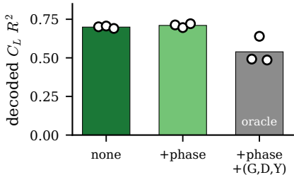
(b) conditioning null (tuned REX, CLW), n=3 operator seeds
