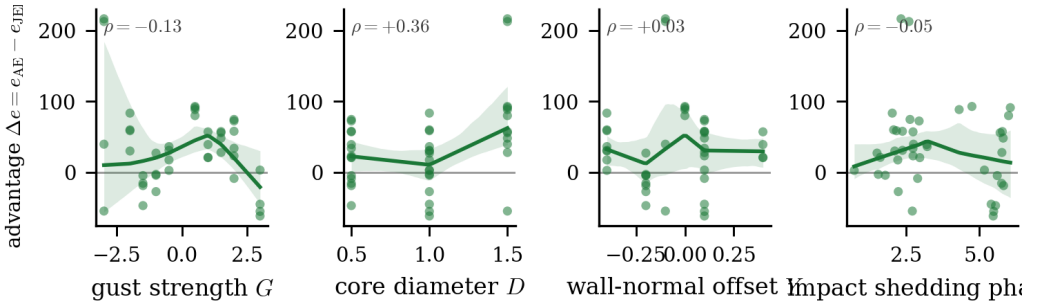
Figure 17. Per-encounter paired improvement \Delta e = e_{AE} - e_{JEPA} in held-out wake-enstrophy error against the gust strength G , core diameter D , wall-normal offset Y , and the baseline shedding phase at impact \phi (test_b, n = 42 ); positive \Delta e means the predictive latent carries the smaller error. Each panel shows the per-encounter values, a locally weighted (LOWESS) trend, and a bootstrap band over encounters. The predictive advantage grows with D (significant) but shows no significant G or Y trend; the shedding-phase axis falls into two clusters because impact is fixed near a single convective instant.
