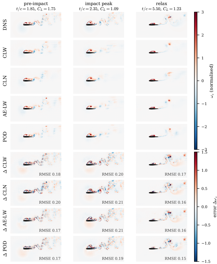
Figure 25. [APA-C11] Decode floor on a representative held-out in-distribution test encounter (one decoder seed per model): DNS, the wake-supervised predictive state, the lift-focused predictive state, the wake autoencoder and the linear basis, and the error rows at three phases. Identical-capacity frozen decoders; normalised vorticity at the fixed \pm 3 range. All four states render the field faithfully, including the linear basis: field decode is not where the states separate.
