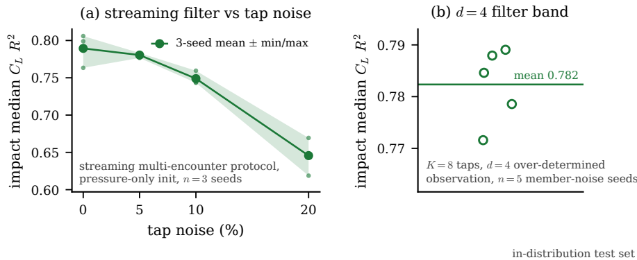
Figure 29. [APB-C2] Deployment realism (in-distribution test set): (a) streaming multi-encounter filter against tap noise, three member-noise seeds, validation-selected band (no test-set reference); (b) the d = 4 filter band over five member-noise seeds.
