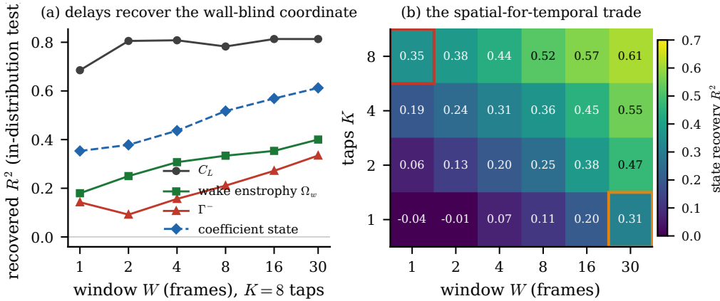
Figure 12. [S4-C3]Sensors traded for delays. (a) Recovery of each observable from eight wall-pressure taps against the length of the pressure window (in-distribution test set); the wall-blind wake circulation rises with the window while the force, visible at one instant, does not. (b) Coefficient-state recovery over the tap-count by window-length grid, with the single-tap, thirty-frame cell and the reference eight-tap, single-frame cell outlined: a long window with few taps matches a short window with many.
