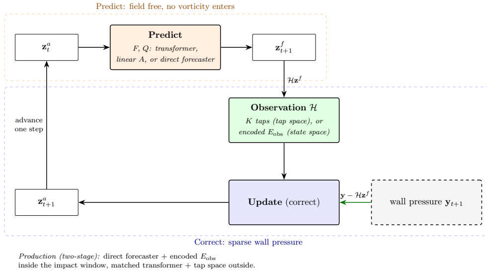
Figure 6. [S34-C1] The predict-correct loop at deployment. An ensemble of 64 members is advanced field free through the matched prediction model, then corrected from 8 span-averaged wall-pressure taps held out from training and placed by the per-model sensor selection. The innovation is the measured minus the predicted observation, formed in tap space for the base filter of §3.3.1 and in encoded latent space for the filters of §3.3.2 and §3.3.3, and the update is a stochastic ensemble Kalman step at inflation \rho = 1 with calibrated \mathbf{Q} and \mathbf{R} . All four estimator configurations are this one loop with only the two annotated slots swapped, the propagation ( F, Q ) and the observation path; table 13 gives the settings per configuration. No vorticity field enters the loop, the state is the same 32-vector at every step, and the lift and wake probes never enter the innovation, which is what makes the reported analysis closure an estimate rather than a quantity the filter was handed.
