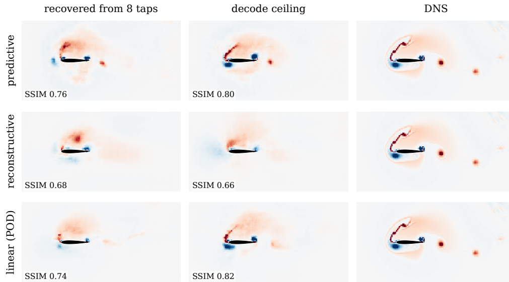
Figure 28. [APB-C1] Flow recovered from eight wall-pressure taps on the representative held-out encounter of figure 13, at the impact-side frame, one row per family. Columns: the field decoded from the pressure-recovered coefficient state, the decode ceiling (the same decoder applied to the encoded state, no pressure step), and the simulation; per-panel structural similarity annotated. The comparison is within each row, since the decoders' ceilings differ (§5.3); the ceiling-to-recovered gap is the cost of the pressure step.
