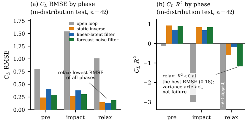
Figure 15. [S4D-C1] Phase-resolved lift tracking with the forecast-noise filter at the production coverage band on the in-distribution test set ( n = 42 encounters, K = 8 taps, delay 10, N = 64 members, every-frame pressure). Lift error per phase in physical units (a) and in R^2 (b) at the val-calibrated band: the relaxation R^2 collapse is a variance artefact, the physical error the honest phase metric. The estimator ladder, its noise calibration and the fixed-lag smoother are in appendix C (figure 32).
