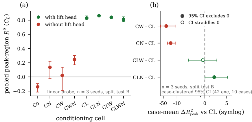
Figure 18. [APA-C4] Paired peak-region lift R^2 per conditioning-cube cell (left) and case-mean deltas against the lift-only cell CL (right, symmetric-log axis, 95 % case-clustered bootstrap intervals over the 42 in-distribution test encounters of 10 cases); filled markers mark intervals that exclude zero. The near-body lift-focused predictive state cell (CLN) is the unique positive increment; the no- L cells sit one to two orders of magnitude lower.
