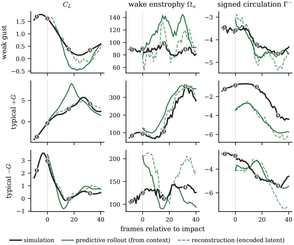
Figure 17. The predictive rollout tracks the encounter, shown qualitatively. Predicted observables through representative held-out encounters (rows), for the lift coefficient, the wake entrophy, and the negative circulation (columns). The simulation is the bold reference; the rollout of the predictor, started from the pre-impact context, is the coloured line, and the dashed line is the reconstruction from the encoded latent. The rollout tracks the wake observables through the leading-edge-vortex peak and into recovery before drifting gently at long times. We report this as qualitative tracking, not as a closure R^2 . Numbered glyphs mark the four encounter stages used throughout: baseline, impact, peak load, and recovery.
