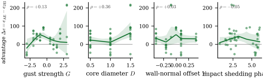
Figure 18. Per-encounter paired improvement \Delta e = e_{AE} - e_{JEPA} in held-out wake-entrophy error against the gust strength G , core diameter D , wall-normal offset Y , and the baseline shedding phase at impact \phi (test_b, n = 42 ); positive \Delta e means the predictive latent carries the smaller error. Each panel shows the per-encounter values, a locally weighted (LOWESS) trend, and a bootstrap band over encounters. The predictive advantage grows with D (significant) but shows no significant G or Y trend; the shedding-phase axis falls into two clusters because impact is fixed near a single convective instant.
