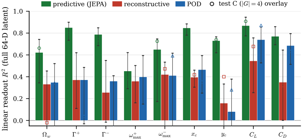
Figure 15. Collective readability of the latent. Held-out test_b R^2 of a single linear readout of the full 64-dimensional latent to each per-frame flow-state descriptor, for the predictive (JEPA), reconstructive (Fukami), and linear (POD) families; error bars are case-clustered bootstrap 95% intervals and the faint open markers are the |G| = 4 extrapolation (test_c). The bars measure how much of each descriptor is linearly available in the whole code, not the semantics of any individual coordinate; the latent is a distributed representation. The gust parameters are omitted as an impact-frame, not a per-frame, quantity.
