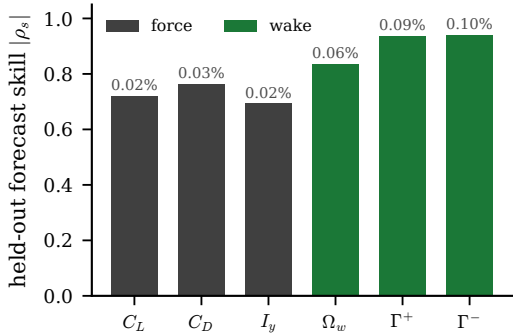
(b) forecast skill per observable
