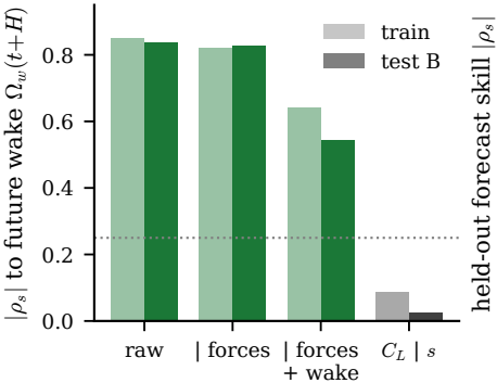
(a) latent wake-forecast signal s
