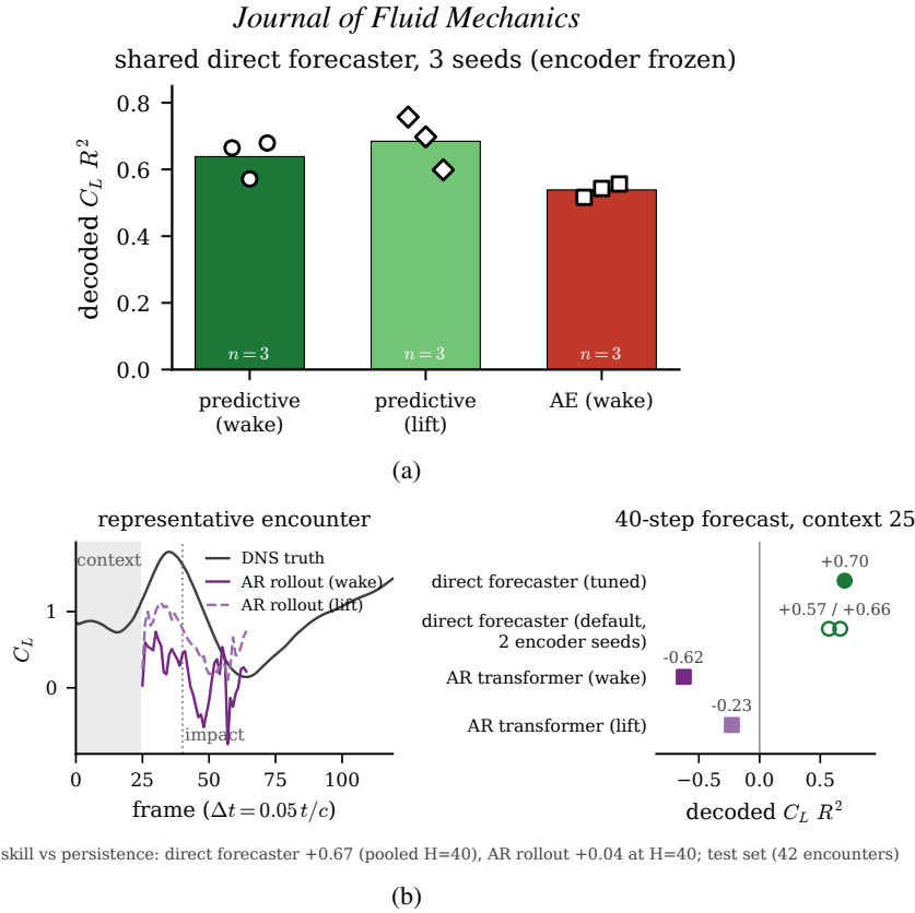
Figure 8. [S4C-C1] Forecasting the state on the in-distribution test set. (a) Decoded lift R^2 of the shared direct multi-horizon forecaster per family (three operator seeds each, the forecaster retrained on a frozen representation, bars at the seed mean): the predictive states forecast the lift best. (b) Direct versus autoregressive over forty steps through the impact from a 25-frame context: the one-shot forecast stays usable where the rollout compounds. The conditioning null, where the (G, D, Y) oracle degrades the forecast and the phase covariate is a wash, is figure 19 in appendix A.
