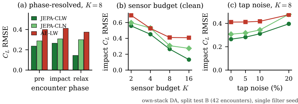
Figure 27. Per-family end-to-end comparison (in-distribution test set, 42 encounters, single filter seed): (a) phase-resolved lift error per family; (b) sensor-budget sweep on each family's own nested placement; (c) tap-noise sweep at K = 8 .
