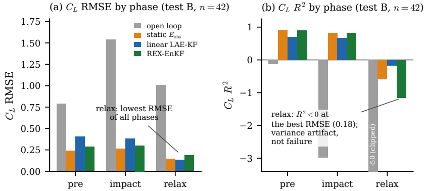
Figure 14. Phase-resolved lift tracking on the in-distribution test set ( n = 42 encounters, K = 8 taps, delay 10, N = 64 members, every-frame pressure). Lift error per phase in physical units (a) and in R^2 (b) at the val-calibrated band: the relaxation R^2 collapse is a variance artifact, the physical error the honest phase metric. The estimator ladder, its noise calibration and the fixed-lag smoother are in appendix C (figure 28).
