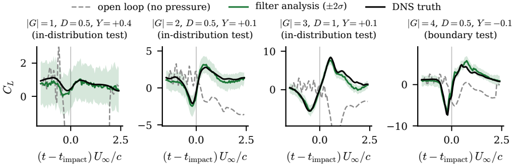
Figure 12. C_L estimation before and after impact across the gust-intensity envelope, on the wake-supervised predictive state ( d = 32 ) under the two-stage filter of §3.3.3: inside the impact window the members are advanced by the direct multi-horizon forecaster’s median forecast with its quantile band as state-dependent process noise (production scale c = 1.77 , validation-calibrated) and corrected by the encoded pressure observation; outside it, by the matched transformer with the tap-space update. Eight wall-pressure taps, N = 64 members; the lift probe that produces the plotted read-out never enters the innovation. Band: \pm 2 ensemble standard deviations; grey, the same stage-scheduled forecast models rolled deterministically without pressure. One representative encounter per |G| stratum (median impact closure on the frozen two-stage filter records; in-distribution test set for |G| \leq 3 , boundary test set at |G| = 4 , where this filter posts no large-error encounter). The analysis tracks the lift through impact and relaxation at every intensity; the open loop loses the transient.
