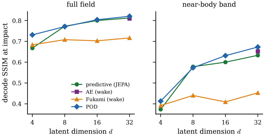
Figure 22. Decode SSIM at the impact instant against latent dimension d (full field and near-body band, in-distribution test set, decode floor). The compact nonlinear states and the linear basis improve with d and saturate together; only the published-recipe lineage plateaus lower. Field decode is not the discriminator at any dimension. Single encoder/decoder seed.
