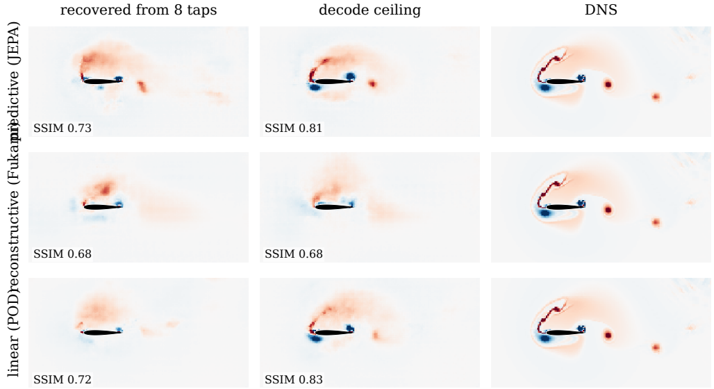
Figure 24. Flow recovered from eight wall-pressure taps on the representative held-out encounter of figure 11, at the impact-side frame, one row per family. Columns: the field decoded from the pressure-recovered coefficient state, the decode ceiling (the same decoder applied to the encoded state, no pressure step), and the simulation; per-panel structural similarity annotated. The comparison is within each row, since the decoders’ ceilings differ (§5.3); the ceiling-to-recovered gap is the cost of the pressure step.
