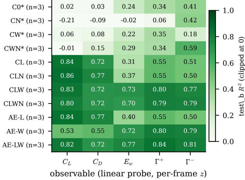
Figure 19. Task-dependent readability (in-distribution test set, linear probes on the per-frame state, seed mean over three encoder seeds per cell): lift and drag follow the L head, the wake block ( E_w , \Gamma^\pm ) follows the W head or the reconstruction objective, and collapsed cells (asterisks) read nothing linearly.
