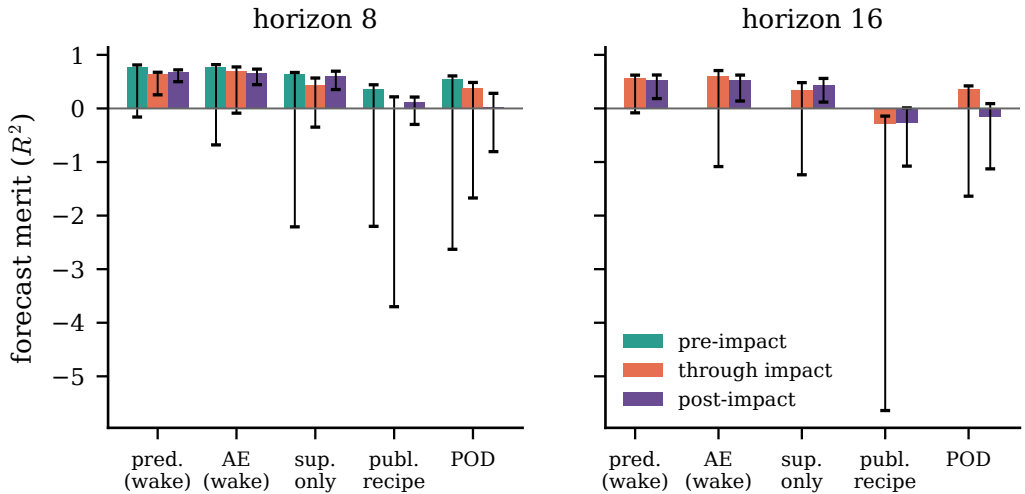
Figure 23. Shared-operator forecast merit split by phase (pre-impact, through-impact, post-impact), per family at horizons eight and sixteen (in-distribution test set, five observables, three operator seeds; bars at the seed mean, case-clustered 95 % intervals). Through-impact merit separates the families: the wake-supervised states hold, the published-recipe reconstruction collapses across the transient, and the linear basis fades into the relaxation.
