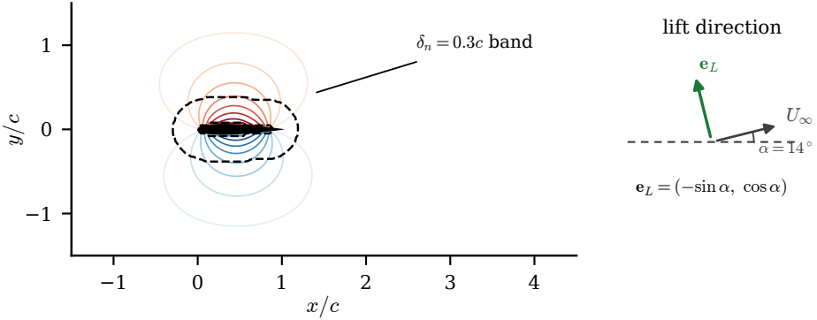
Figure 20. The Chang auxiliary potential \phi_L of equation (3.1) on the cache grid (contours), the feathered \delta_n = 0.3c supervision band (dashed) and the airfoil footprint; the inset shows the lift direction \mathbf{e}_L against the inclined freestream at \alpha = 14^\circ .
