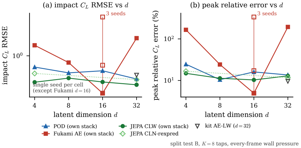
Figure 13. The assimilation-versus-dimension grid (in-distribution test set, per-family end-to-end stacks, K = 8 , every-frame pressure; single seed per cell except the reconstructive d = 16 cell, which carries three): impact error and relative peak error against dimension for the three families. The predictive family is uniform, the linear basis stable, the reconstructive baseline non-monotonic in dimension and irreproducible across seeds.
